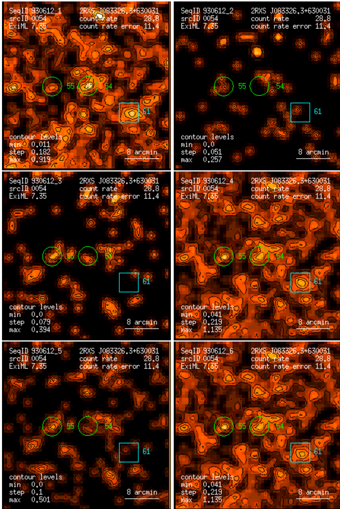
Figure 54: RASS 930612: detection 0054: band rate images, Gaussian filter: (1) PSPC channels 11 – 41, (2) 52 – 90, (3) 91 – 201, (4) 11 – 235, (5) 52 – 201, (6) 11 – 201. Broad band rates in counts/ks. Band rate contour levels in counts/ks/arcmin 2 .
