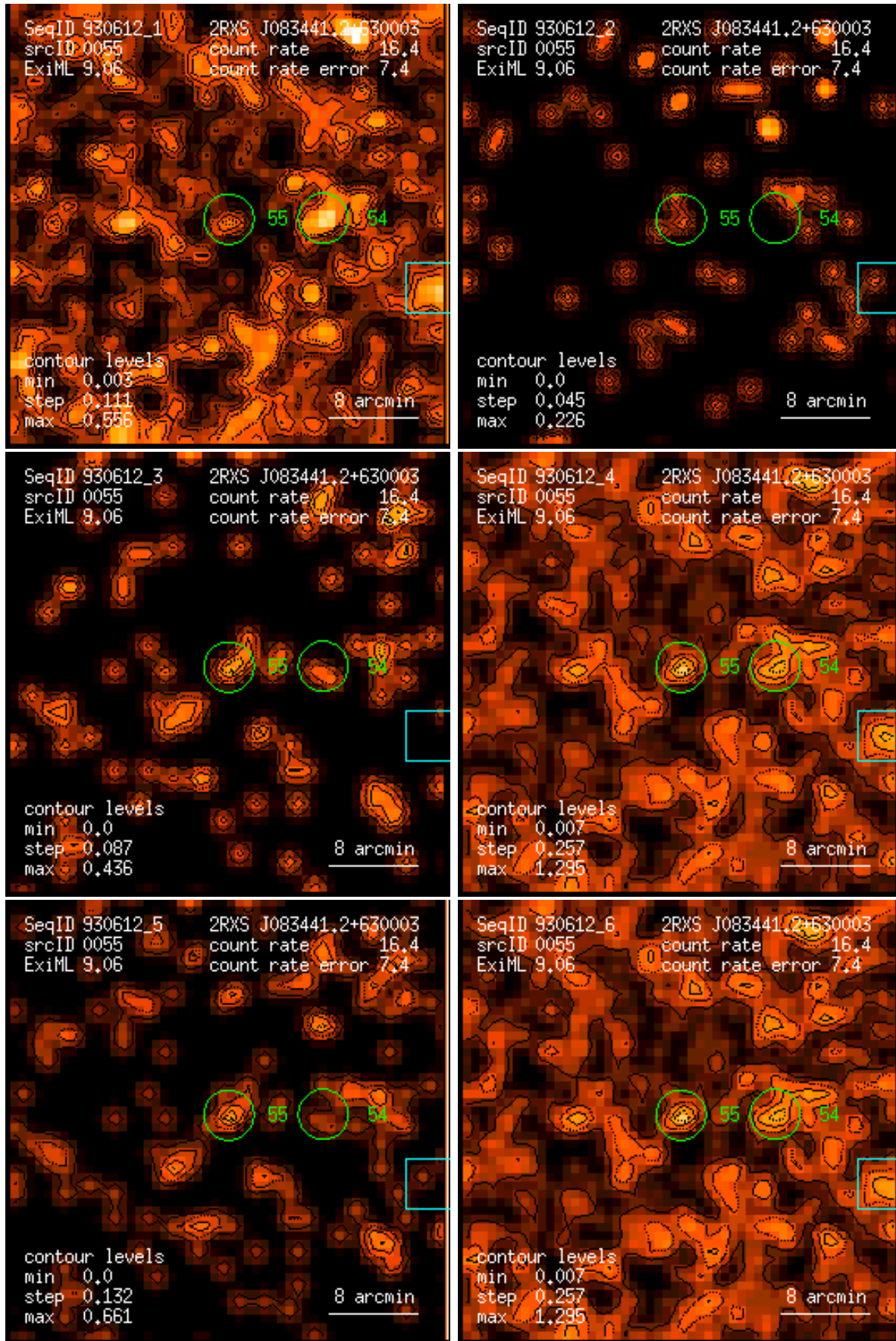
Figure 55: RASS 930612: detection 0055: band rate images, Gaussian filter: (1) PSPC channels 11 – 41, (2) 52 – 90, (3) 91 – 201, (4) 11 – 235, (5) 52 – 201, (6) 11 – 201. Broad band rates in counts/ks. Band rate contour levels in counts/ks/arcmin 2 .
