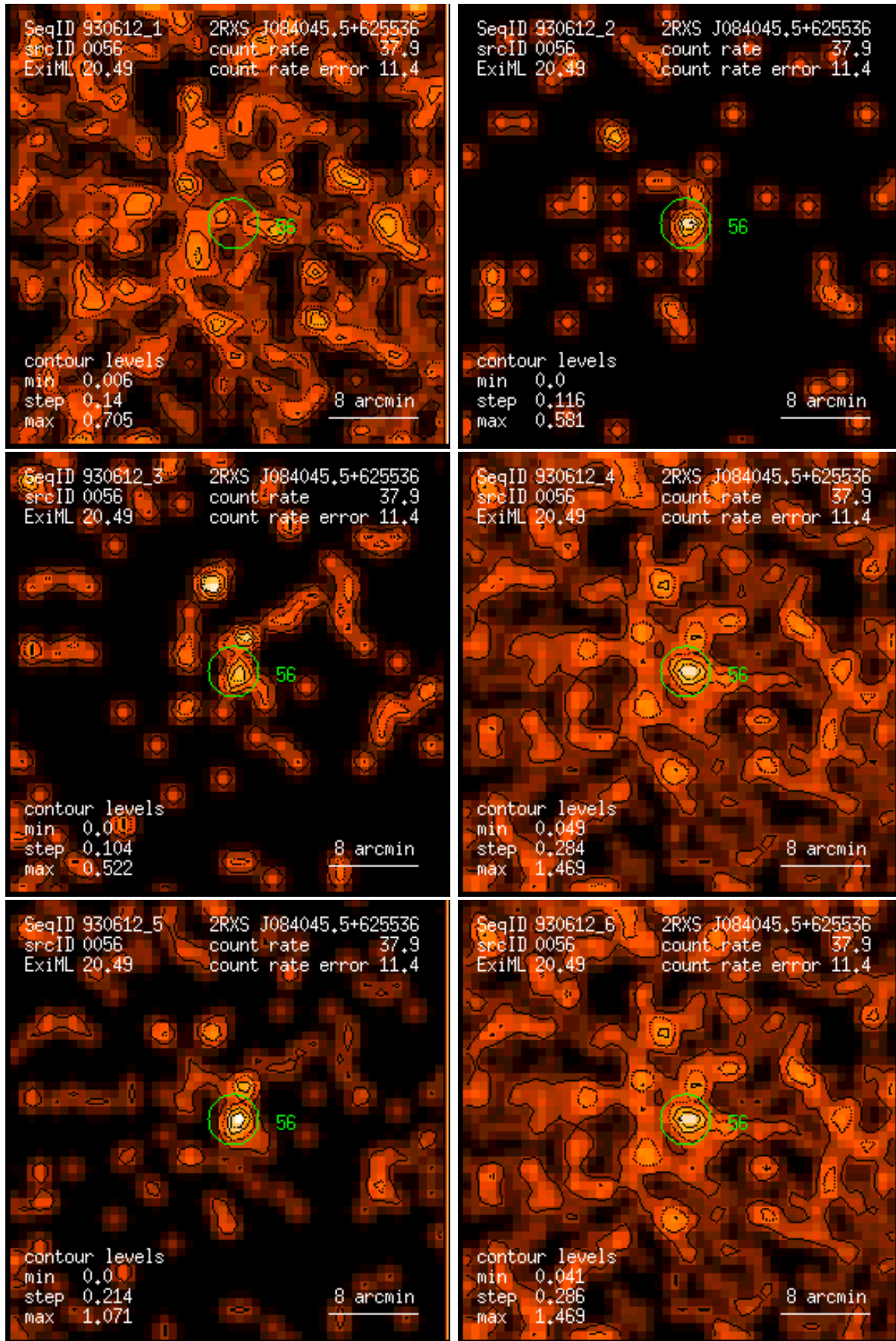
Figure 56: RASS 930612: detection 0056: band rate images, Gaussian filter: (1) PSPC channels 11 – 41, (2) 52 – 90, (3) 91 – 201, (4) 11 – 235, (5) 52 – 201, (6) 11 – 201. Broad band rates in counts/ks. Band rate contour levels in counts/ks/arcmin 2 .
