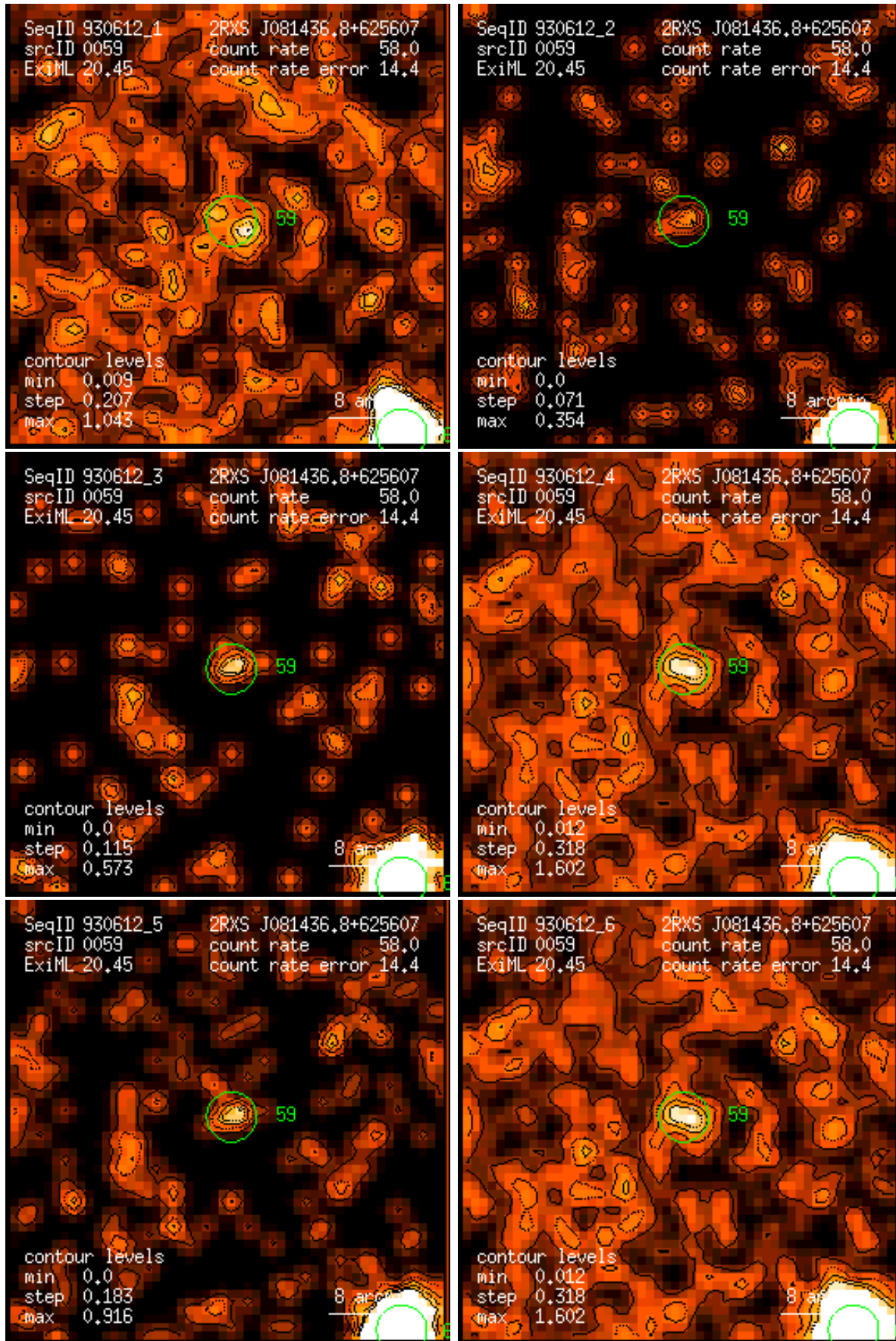
Figure 59: RASS 930612: detection 0059: band rate images, Gaussian filter: (1) PSPC channels 11 – 41, (2) 52 – 90, (3) 91 – 201, (4) 11 – 235, (5) 52 – 201, (6) 11 – 201. Broad band rates in counts/ks. Band rate contour levels in counts/ks/arcmin 2 .
