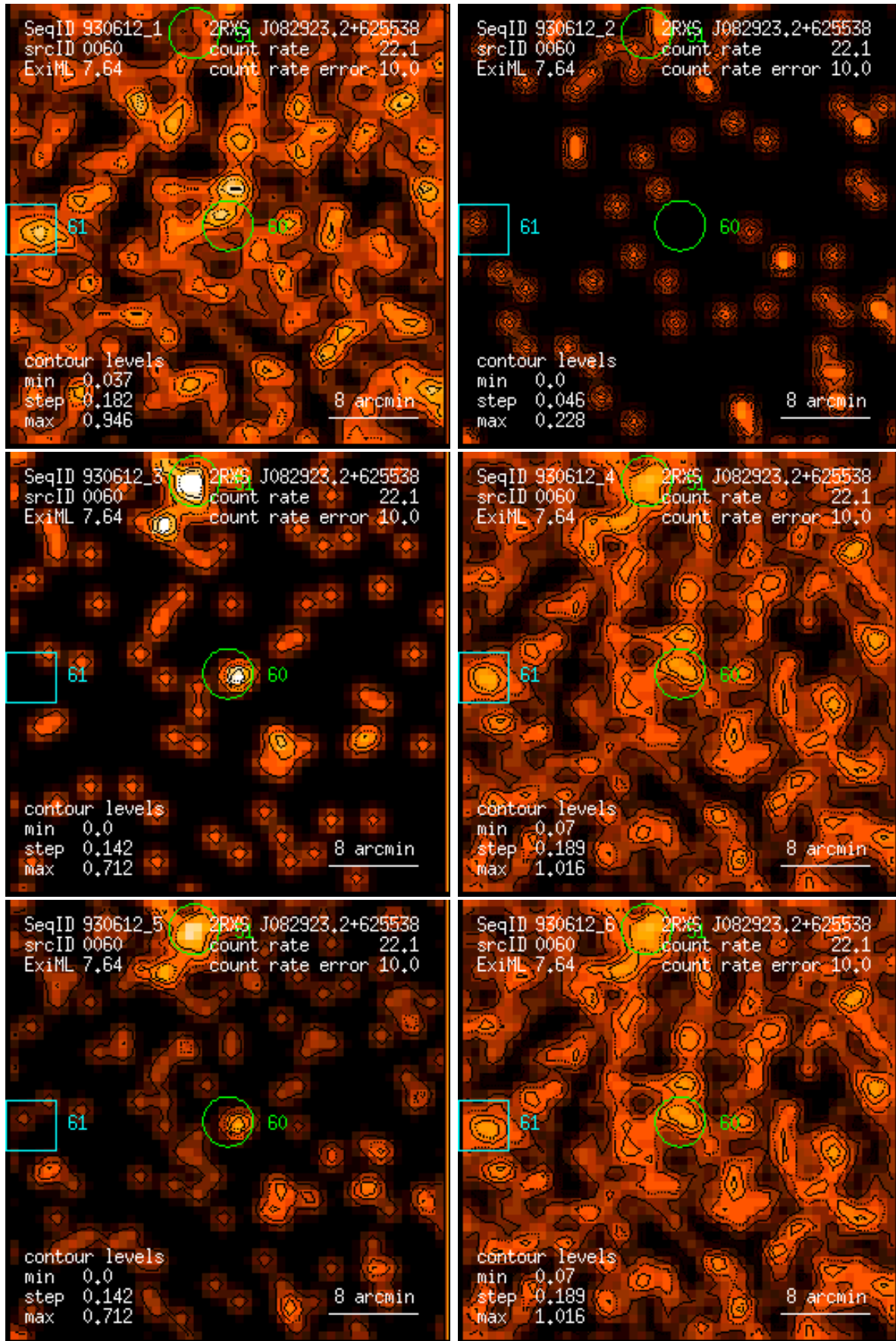
Figure 60: RASS 930612: detection 0060: band rate images, Gaussian filter: (1) PSPC channels 11 – 41, (2) 52 – 90, (3) 91 – 201, (4) 11 – 235, (5) 52 – 201, (6) 11 – 201. Broad band rates in counts/ks. Band rate contour levels in counts/ks/arcmin 2 .
