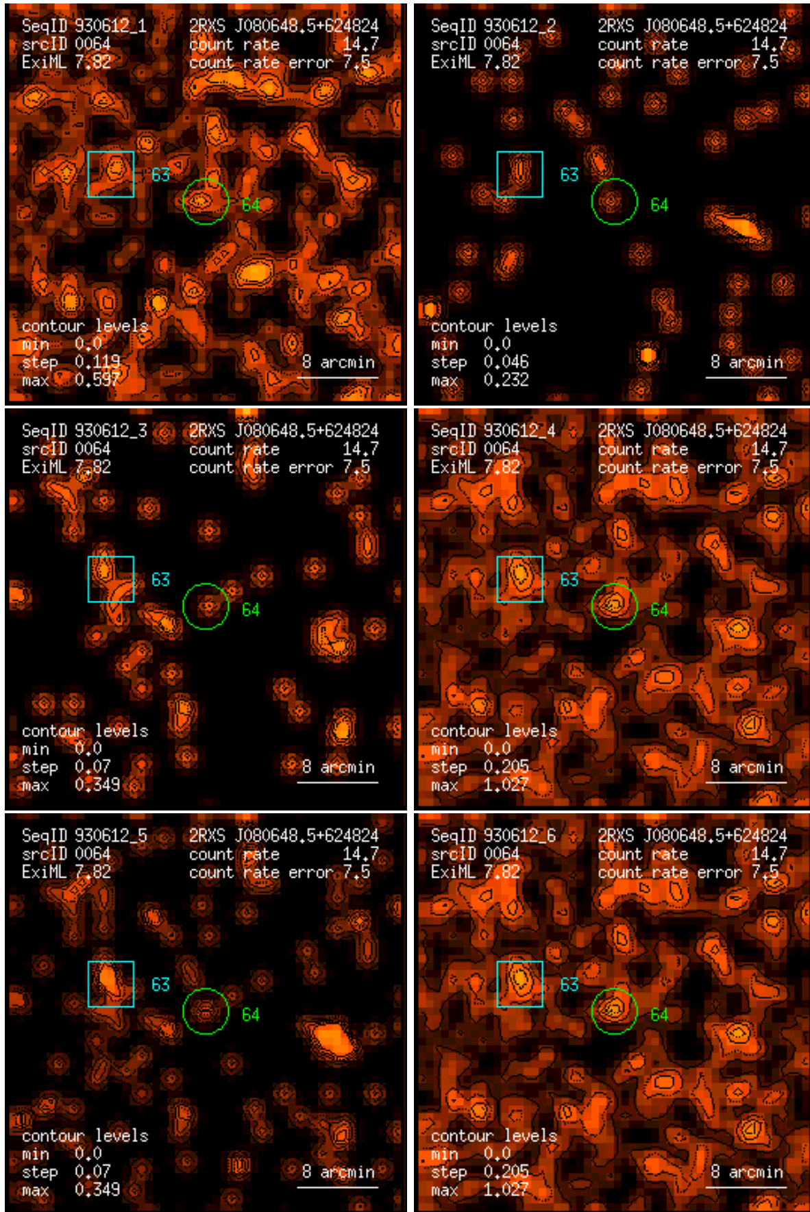
Figure 64: RASS 930612: detection 0064: band rate images, Gaussian filter: (1) PSPC channels 11 – 41, (2) 52 – 90, (3) 91 – 201, (4) 11 – 235, (5) 52 – 201, (6) 11 – 201. Broad band rates in counts/ks. Band rate contour levels in counts/ks/arcmin 2 .
