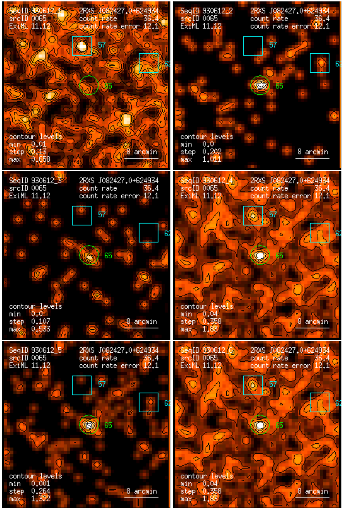
Figure 65: RASS 930612: detection 0065: band rate images, Gaussian filter: (1) PSPC channels 11 – 41, (2) 52 – 90, (3) 91 – 201, (4) 11 – 235, (5) 52 – 201, (6) 11 – 201. Broad band rates in counts/ks. Band rate contour levels in counts/ks/arcmin 2 .
