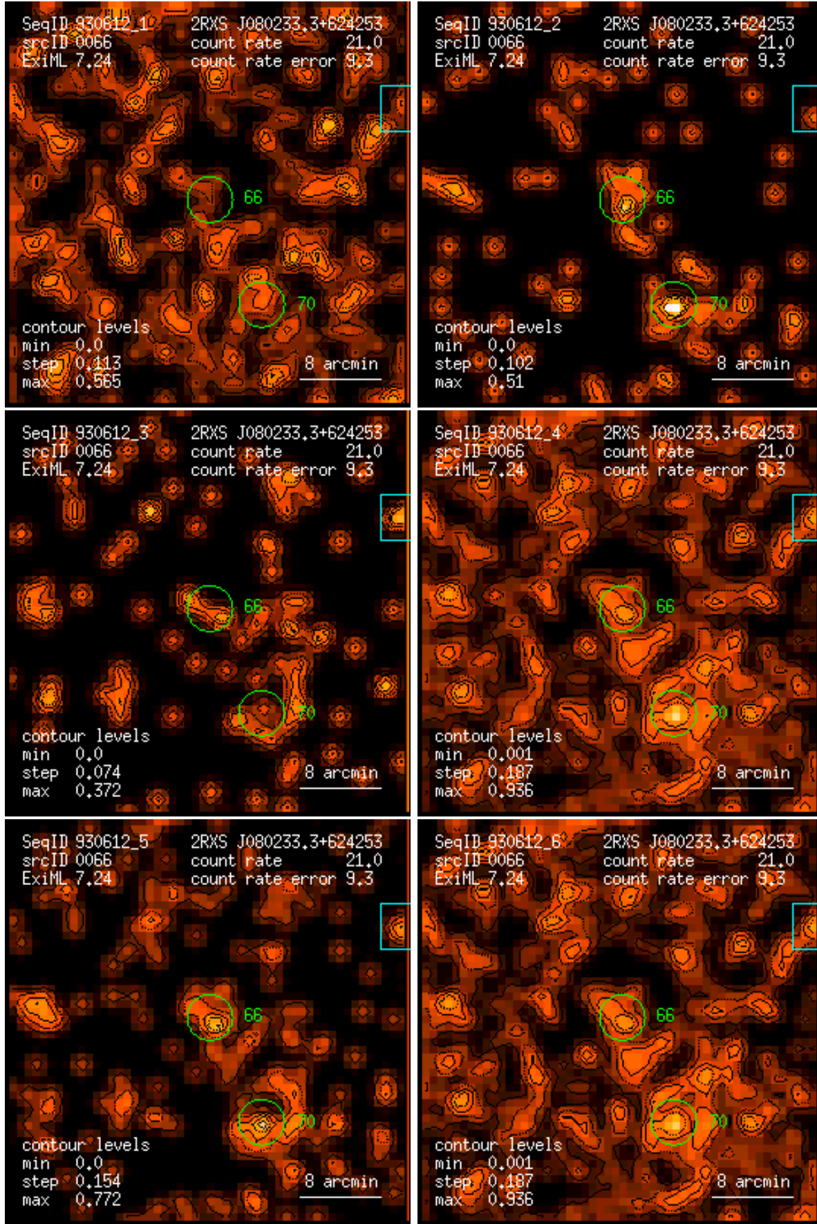
Figure 66: RASS 930612: detection 0066: band rate images, Gaussian filter: (1) PSPC channels 11 – 41, (2) 52 – 90, (3) 91 – 201, (4) 11 – 235, (5) 52 – 201, (6) 11 – 201. Broad band rates in counts/ks. Band rate contour levels in counts/ks/arcmin 2 .
