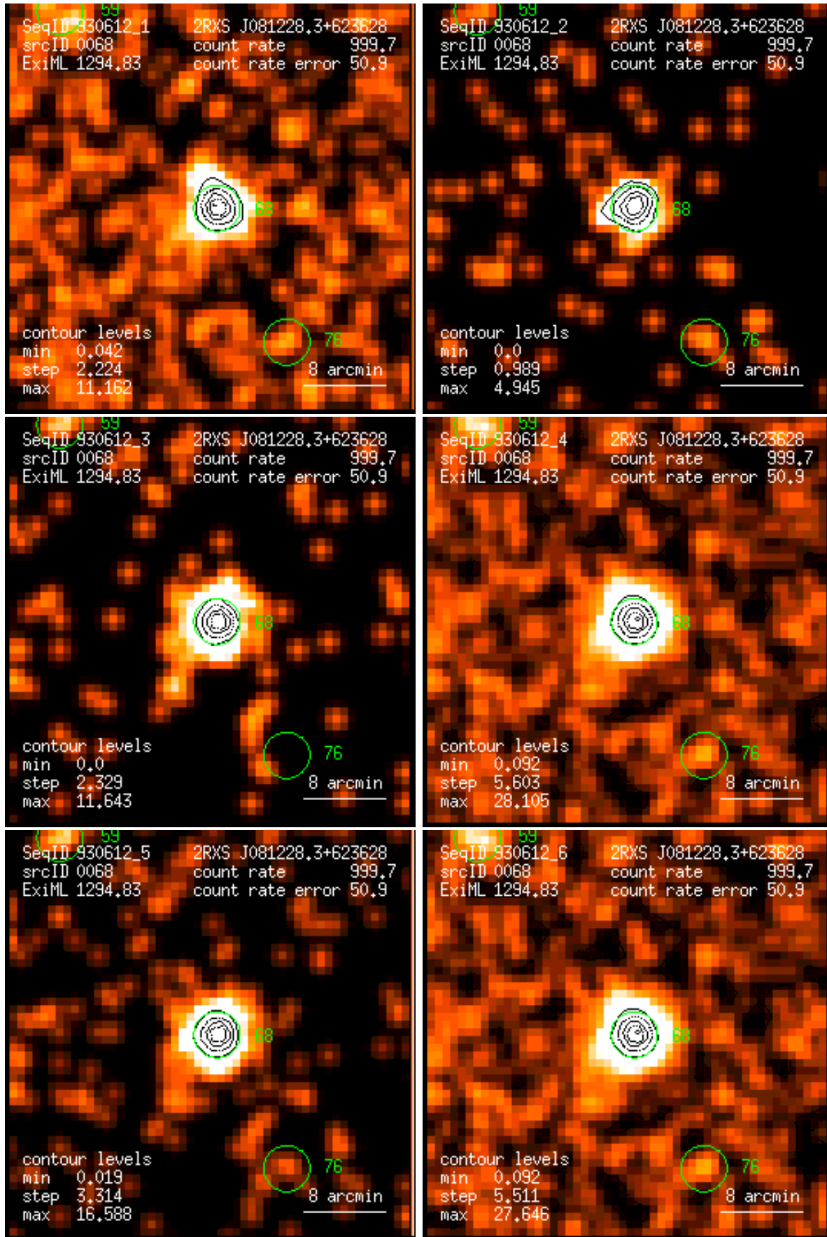
Figure 68: RASS 930612: detection 0068: band rate images, Gaussian filter: (1) PSPC channels 11 – 41, (2) 52 – 90, (3) 91 – 201, (4) 11 – 235, (5) 52 – 201, (6) 11 – 201. Broad band rates in counts/ks. Band rate contour levels in counts/ks/arcmin 2 .
