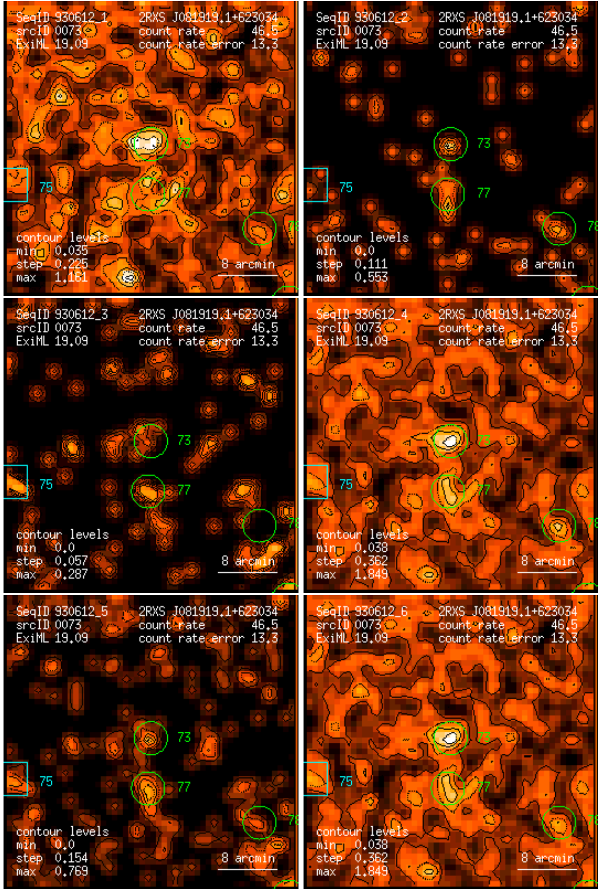
Figure 73: RASS 930612: detection 0073: band rate images, Gaussian filter: (1) PSPC channels 11 – 41, (2) 52 – 90, (3) 91 – 201, (4) 11 – 235, (5) 52 – 201, (6) 11 – 201. Broad band rates in counts/ks. Band rate contour levels in counts/ks/arcmin 2 .
