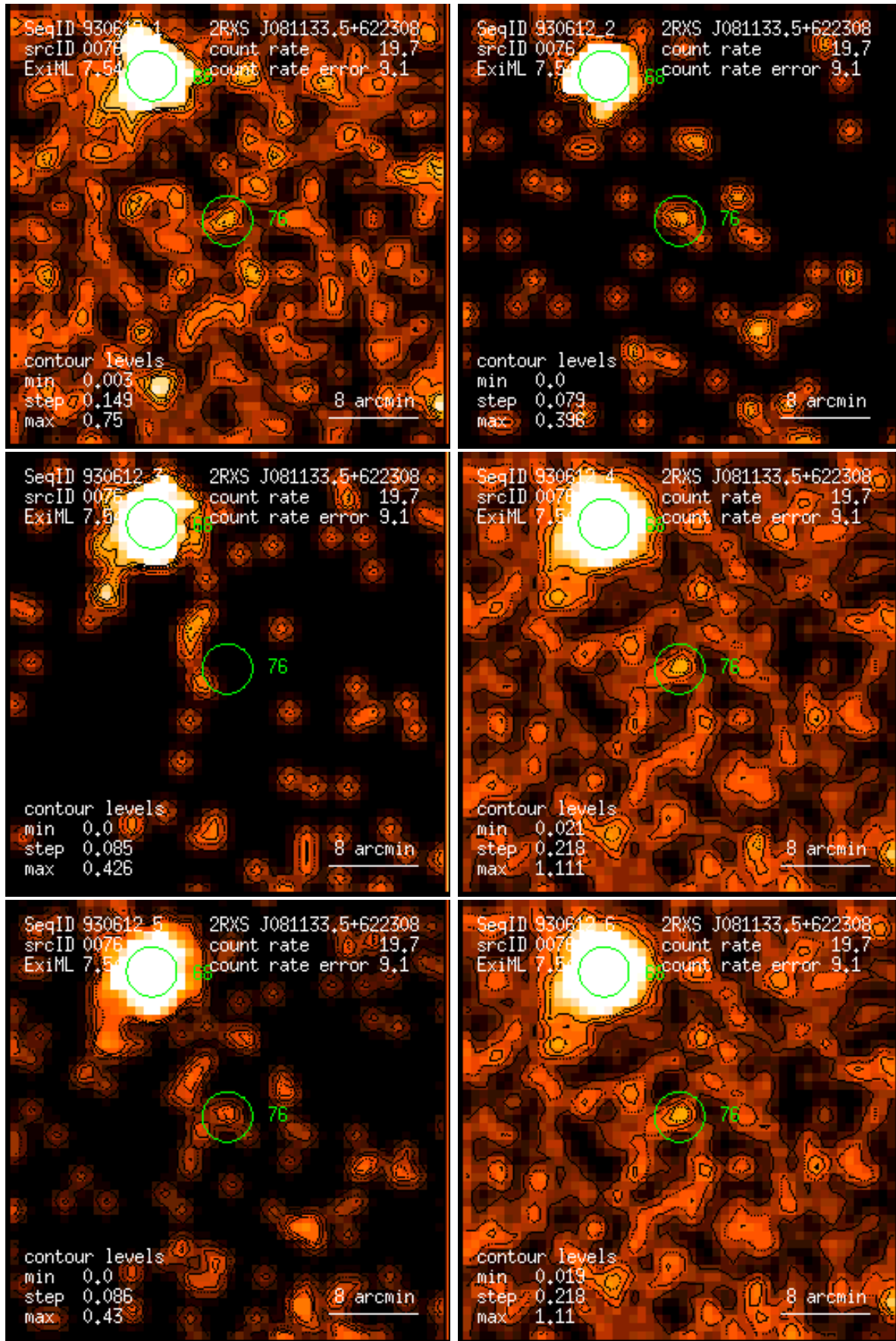
Figure 76: RASS 930612: detection 0076: band rate images, Gaussian filter: (1) PSPC channels 11 – 41, (2) 52 – 90, (3) 91 – 201, (4) 11 – 235, (5) 52 – 201, (6) 11 – 201. Broad band rates in counts/ks. Band rate contour levels in counts/ks/arcmin 2 .
