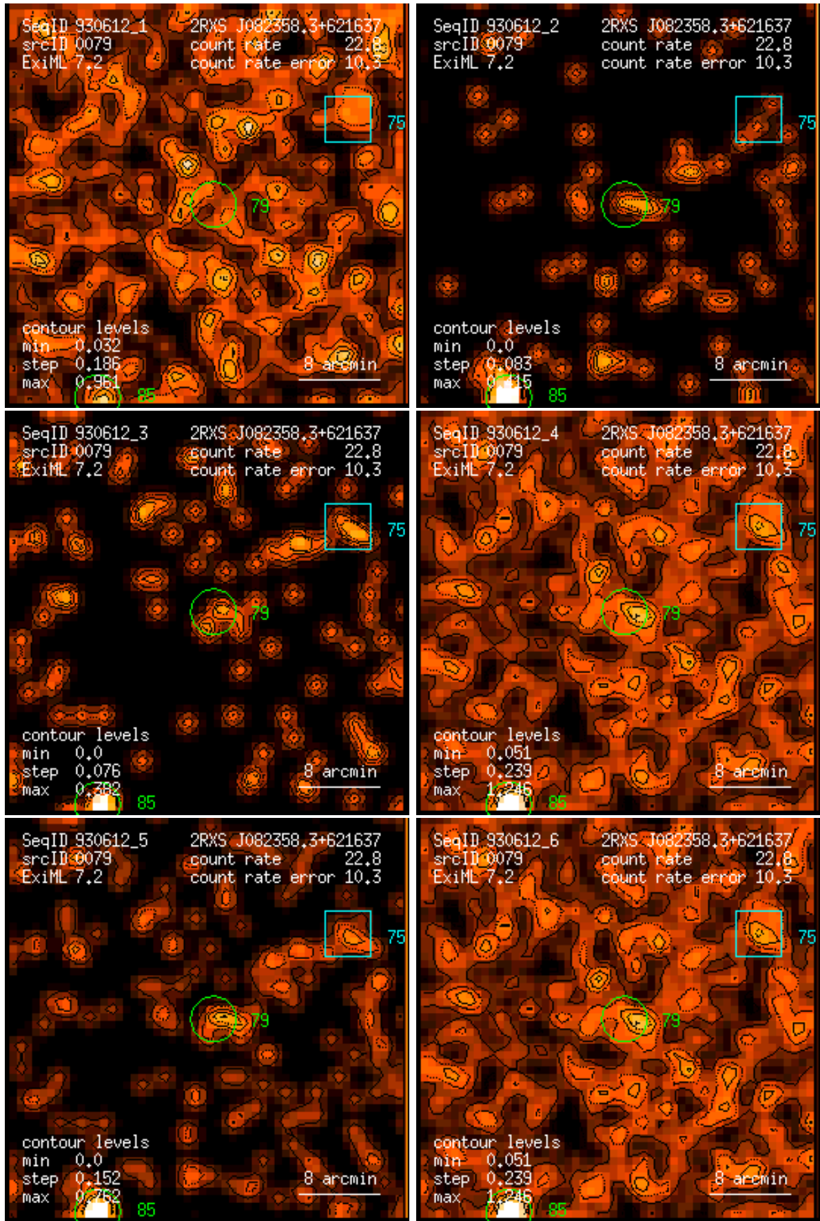
Figure 79: RASS 930612: detection 0079: band rate images, Gaussian filter: (1) PSPC channels 11 – 41, (2) 52 – 90, (3) 91 – 201, (4) 11 – 235, (5) 52 – 201, (6) 11 – 201. Broad band rates in counts/ks. Band rate contour levels in counts/ks/arcmin 2 .
