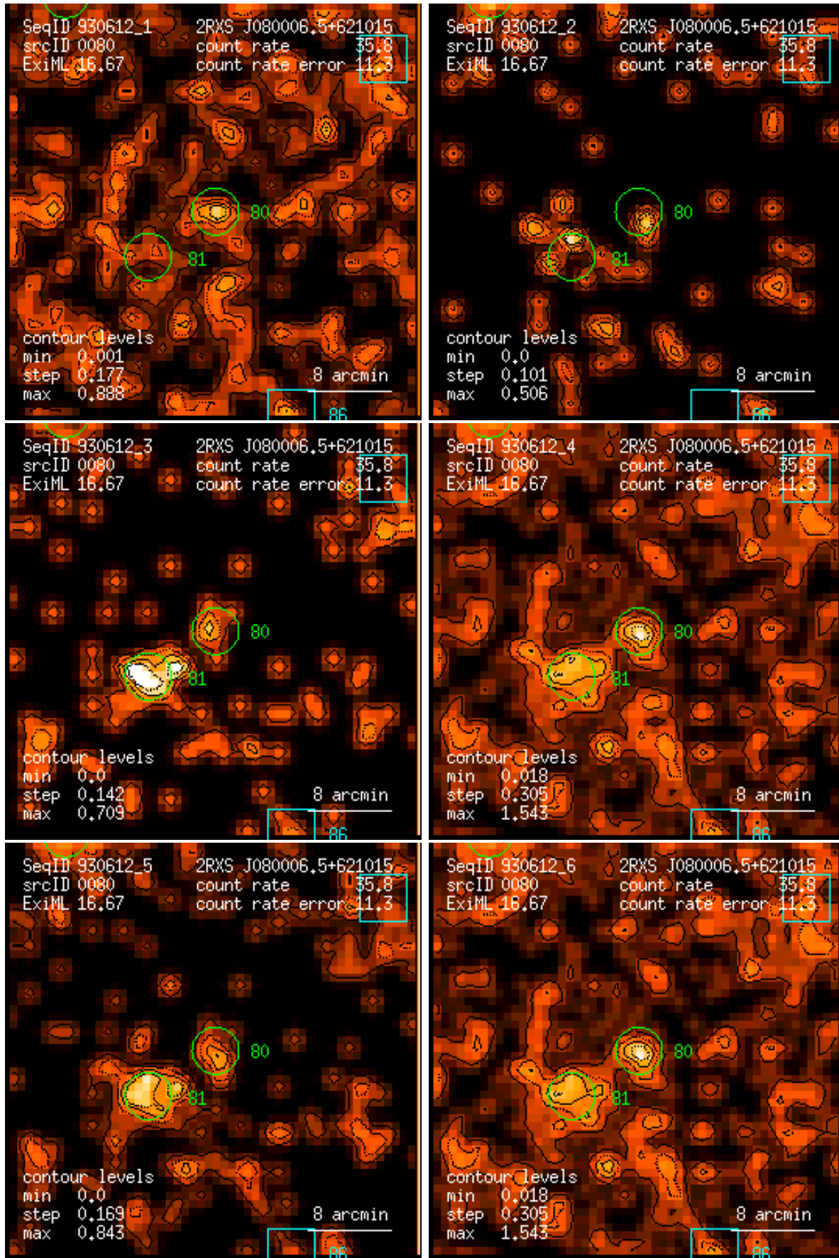
Figure 80: RASS 930612: detection 0080: band rate images, Gaussian filter: (1) PSPC channels 11 – 41, (2) 52 – 90, (3) 91 – 201, (4) 11 – 235, (5) 52 – 201, (6) 11 – 201. Broad band rates in counts/ks. Band rate contour levels in counts/ks/arcmin 2 .
