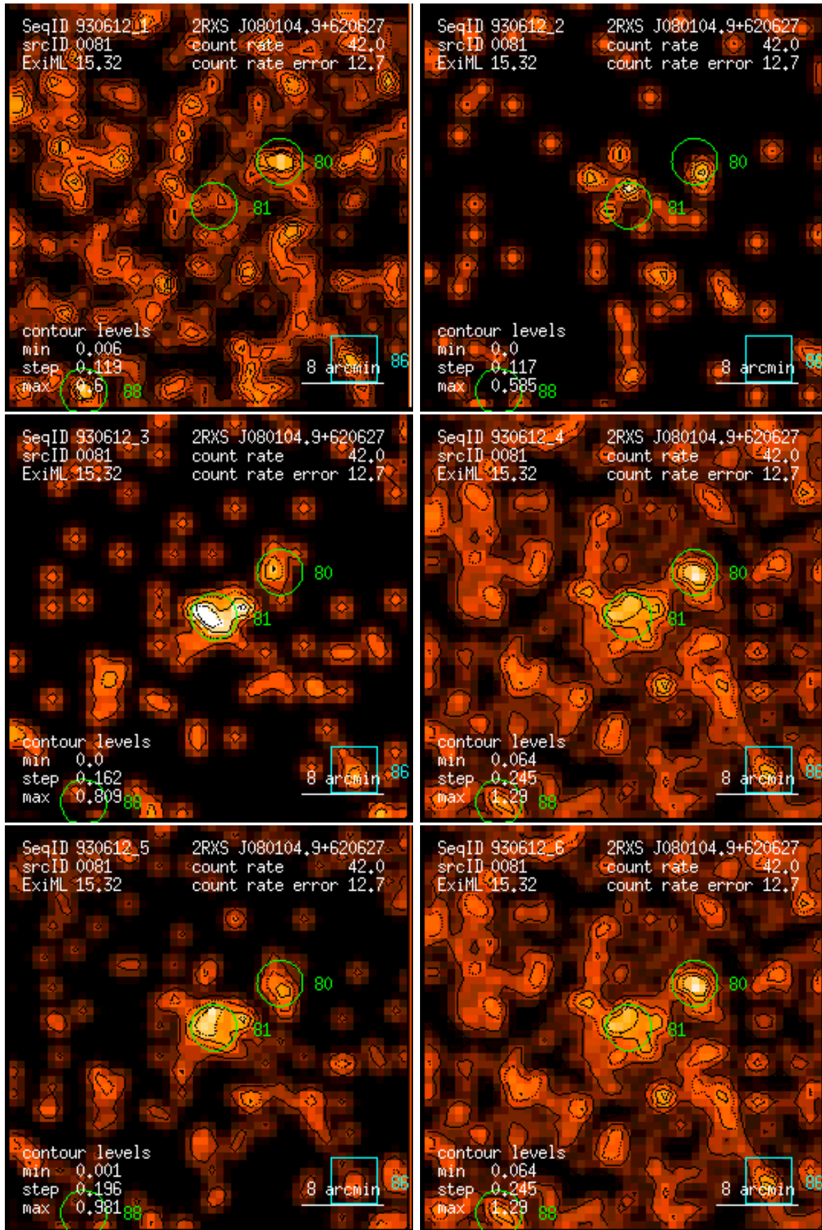
Figure 81: RASS 930612: detection 0081: band rate images, Gaussian filter: (1) PSPC channels 11 – 41, (2) 52 – 90, (3) 91 – 201, (4) 11 – 235, (5) 52 – 201, (6) 11 – 201. Broad band rates in counts/ks. Band rate contour levels in counts/ks/arcmin 2 .
