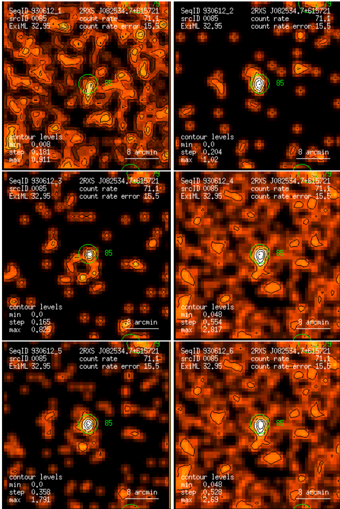
Figure 85: RASS 930612: detection 0085: band rate images, Gaussian filter: (1) PSPC channels 11 – 41, (2) 52 – 90, (3) 91 – 201, (4) 11 – 235, (5) 52 – 201, (6) 11 – 201. Broad band rates in counts/ks. Band rate contour levels in counts/ks/arcmin 2 .
