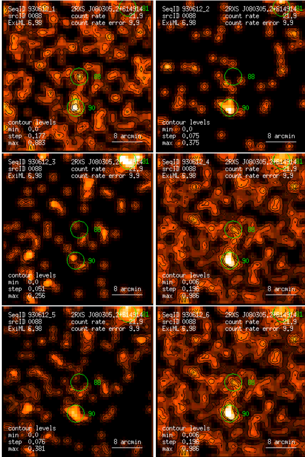
Figure 88: RASS 930612: detection 0088: band rate images, Gaussian filter: (1) PSPC channels 11 – 41, (2) 52 – 90, (3) 91 – 201, (4) 11 – 235, (5) 52 – 201, (6) 11 – 201. Broad band rates in counts/ks. Band rate contour levels in counts/ks/arcmin 2 .
