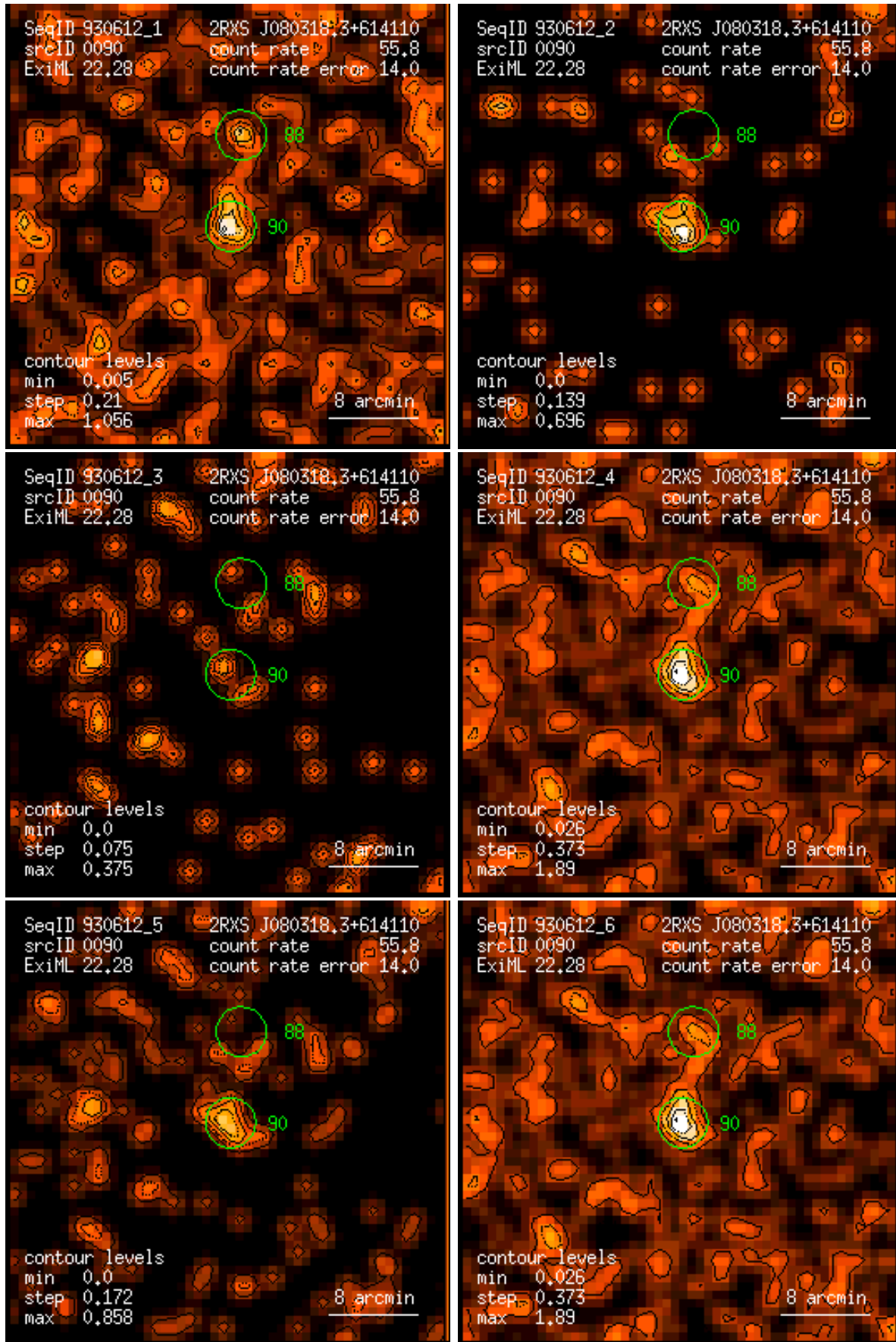
Figure 90: RASS 930612: detection 0090: band rate images, Gaussian filter: (1) PSPC channels 11 – 41, (2) 52 – 90, (3) 91 – 201, (4) 11 – 235, (5) 52 – 201, (6) 11 – 201. Broad band rates in counts/ks. Band rate contour levels in counts/ks/arcmin 2 .
