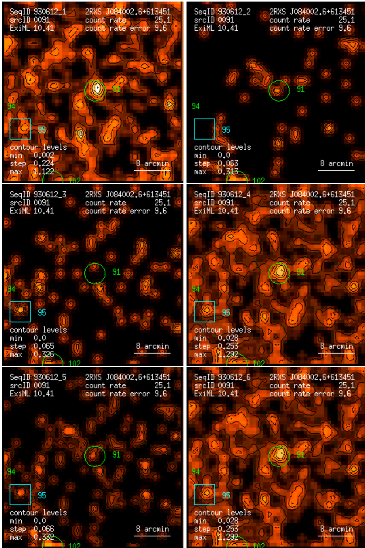
Figure 91: RASS 930612: detection 0091: band rate images, Gaussian filter: (1) PSPC channels 11 – 41, (2) 52 – 90, (3) 91 – 201, (4) 11 – 235, (5) 52 – 201, (6) 11 – 201. Broad band rates in counts/ks. Band rate contour levels in counts/ks/arcmin 2 .
