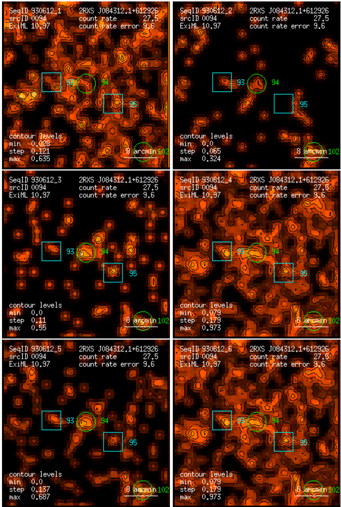
Figure 94: RASS 930612: detection 0094: band rate images, Gaussian filter: (1) PSPC channels 11 – 41, (2) 52 – 90, (3) 91 – 201, (4) 11 – 235, (5) 52 – 201, (6) 11 – 201. Broad band rates in counts/ks. Band rate contour levels in counts/ks/arcmin 2 .
