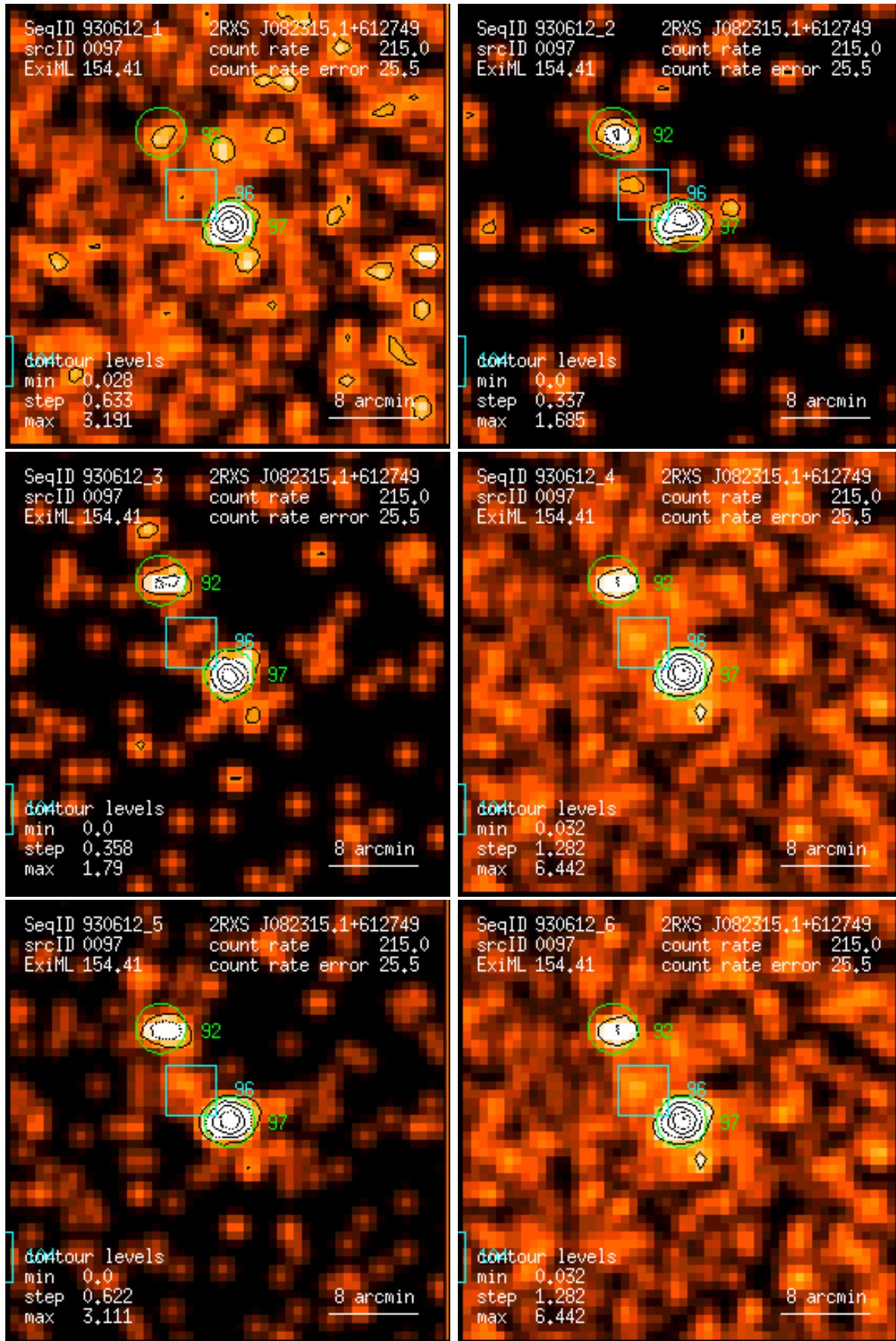
Figure 97: RASS 930612: detection 0097: band rate images, Gaussian filter: (1) PSPC channels 11 – 41, (2) 52 – 90, (3) 91 – 201, (4) 11 – 235, (5) 52 – 201, (6) 11 – 201. Broad band rates in counts/ks. Band rate contour levels in counts/ks/arcmin 2 .
