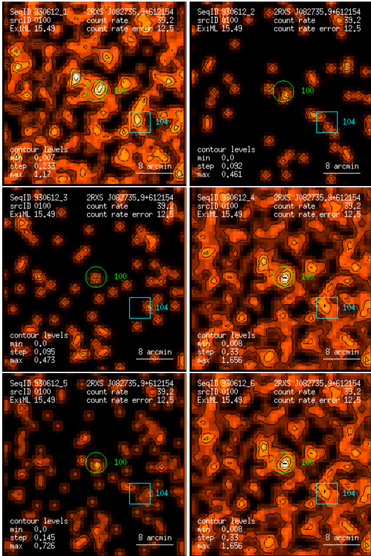
Figure 100: RASS 930612: detection 0100: band rate images, Gaussian filter: (1) PSPC channels 11 – 41, (2) 52 – 90, (3) 91 – 201, (4) 11 – 235, (5) 52 – 201, (6) 11 – 201. Broad band rates in counts/ks. Band rate contour levels in counts/ks/arcmin 2 .
