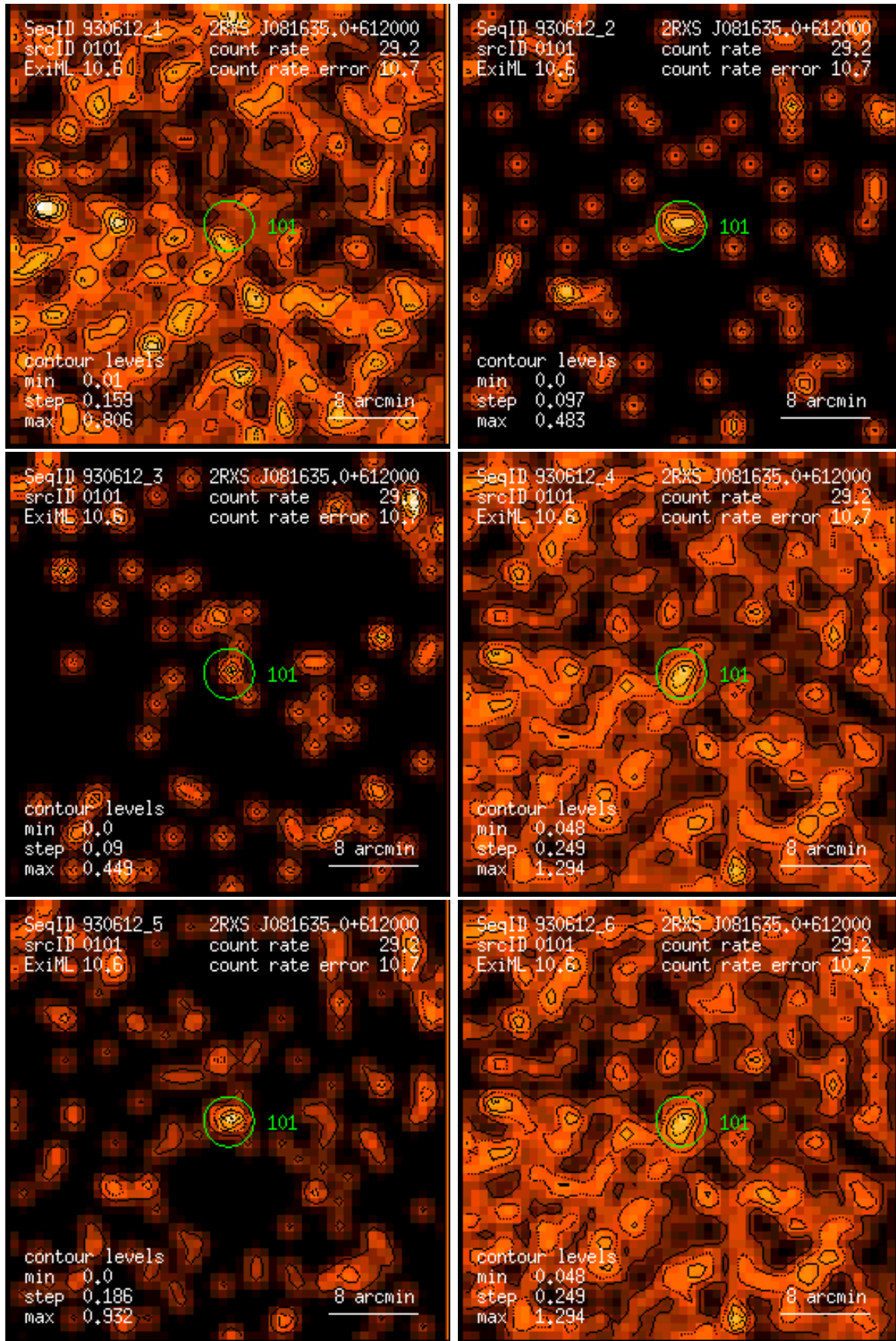
Figure 101: RASS 930612: detection 0101: band rate images, Gaussian filter: (1) PSPC channels 11 – 41, (2) 52 – 90, (3) 91 – 201, (4) 11 – 235, (5) 52 – 201, (6) 11 – 201. Broad band rates in counts/ks. Band rate contour levels in counts/ks/arcmin 2 .
