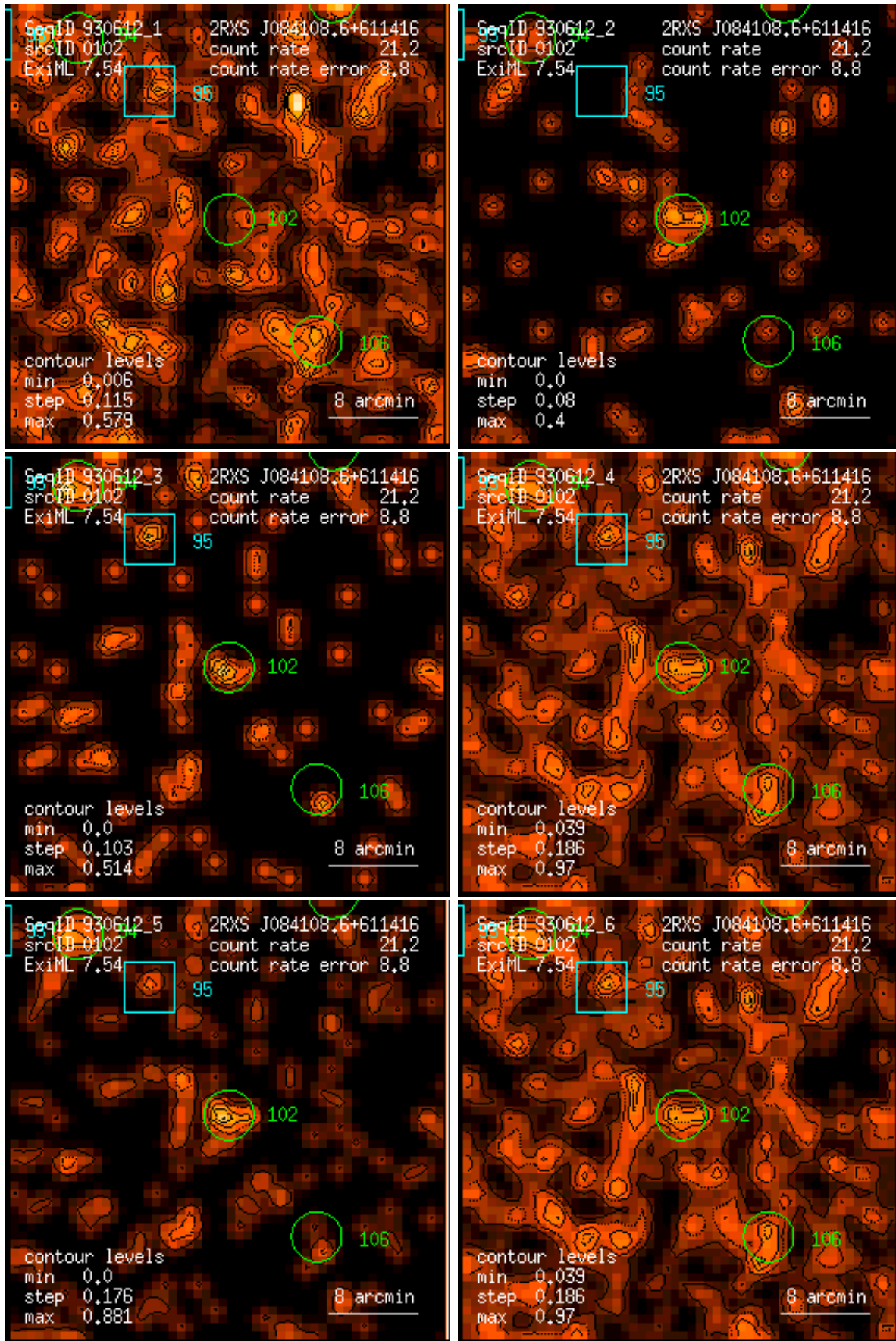
Figure 102: RASS 930612: detection 0102: band rate images, Gaussian filter: (1) PSPC channels 11 – 41, (2) 52 – 90, (3) 91 – 201, (4) 11 – 235, (5) 52 – 201, (6) 11 – 201. Broad band rates in counts/ks. Band rate contour levels in counts/ks/arcmin 2 .
