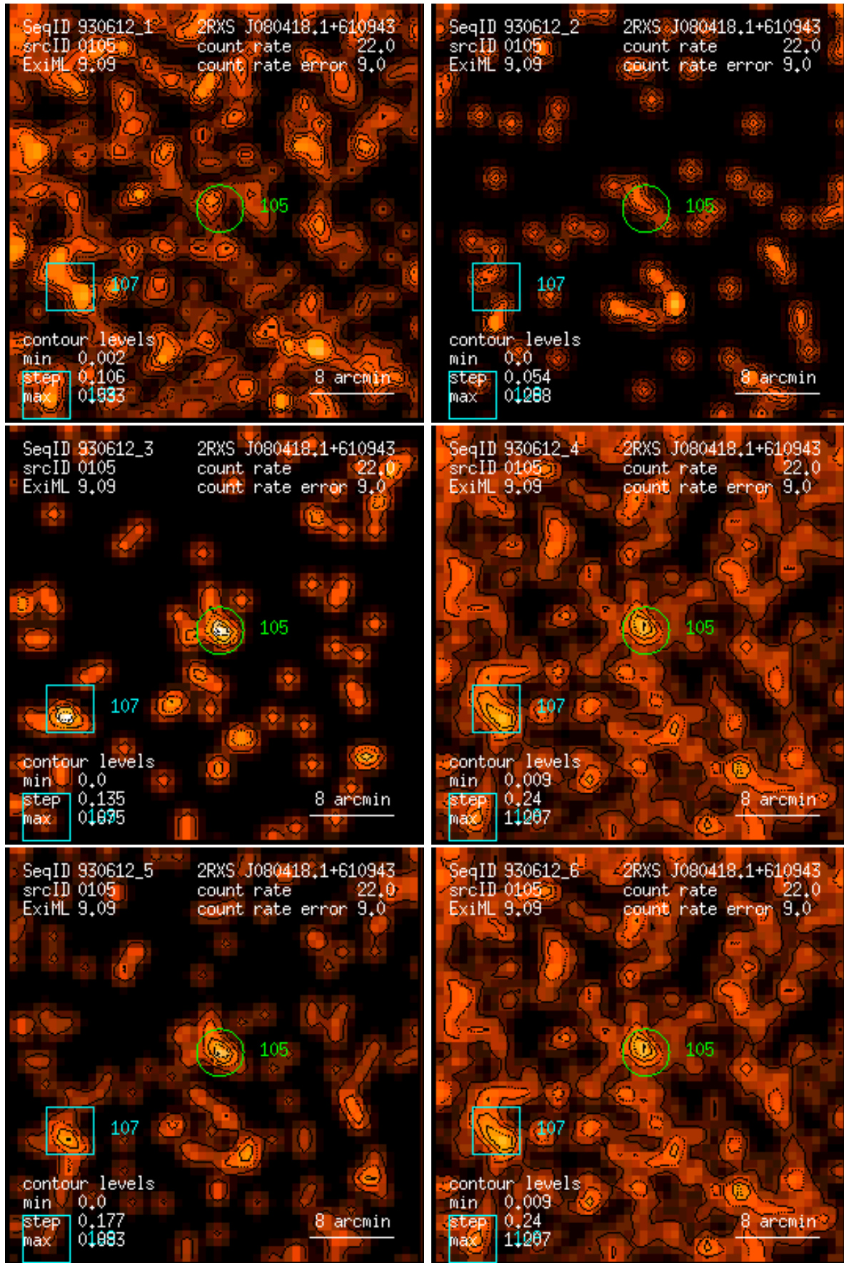
Figure 105: RASS 930612: detection 0105: band rate images, Gaussian filter: (1) PSPC channels 11 – 41, (2) 52 – 90, (3) 91 – 201, (4) 11 – 235, (5) 52 – 201, (6) 11 – 201. Broad band rates in counts/ks. Band rate contour levels in counts/ks/arcmin 2 .
