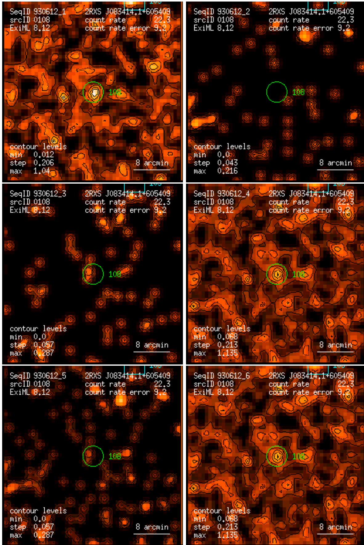
Figure 108: RASS 930612: detection 0108: band rate images, Gaussian filter: (1) PSPC channels 11 – 41, (2) 52 – 90, (3) 91 – 201, (4) 11 – 235, (5) 52 – 201, (6) 11 – 201. Broad band rates in counts/ks. Band rate contour levels in counts/ks/arcmin 2 .
