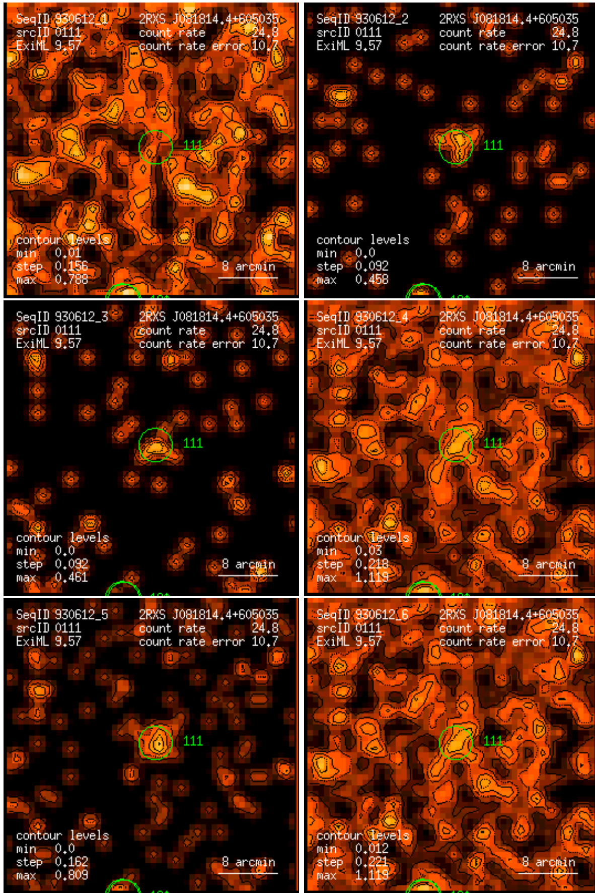
Figure 111: RASS 930612: detection 0111: band rate images, Gaussian filter: (1) PSPC channels 11 – 41, (2) 52 – 90, (3) 91 – 201, (4) 11 – 235, (5) 52 – 201, (6) 11 – 201. Broad band rates in counts/ks. Band rate contour levels in counts/ks/arcmin 2 .
