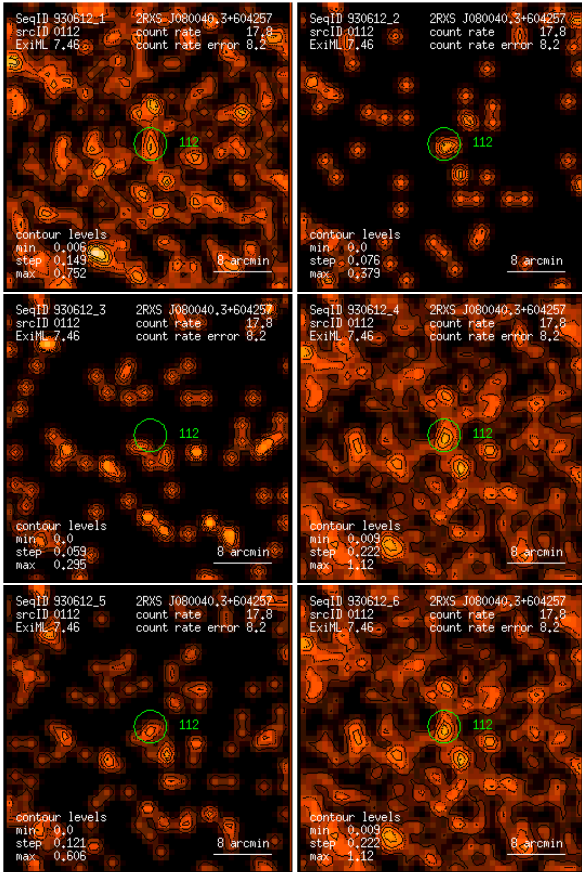
Figure 112: RASS 930612: detection 0112: band rate images, Gaussian filter: (1) PSPC channels 11 – 41, (2) 52 – 90, (3) 91 – 201, (4) 11 – 235, (5) 52 – 201, (6) 11 – 201. Broad band rates in counts/ks. Band rate contour levels in counts/ks/arcmin 2 .
