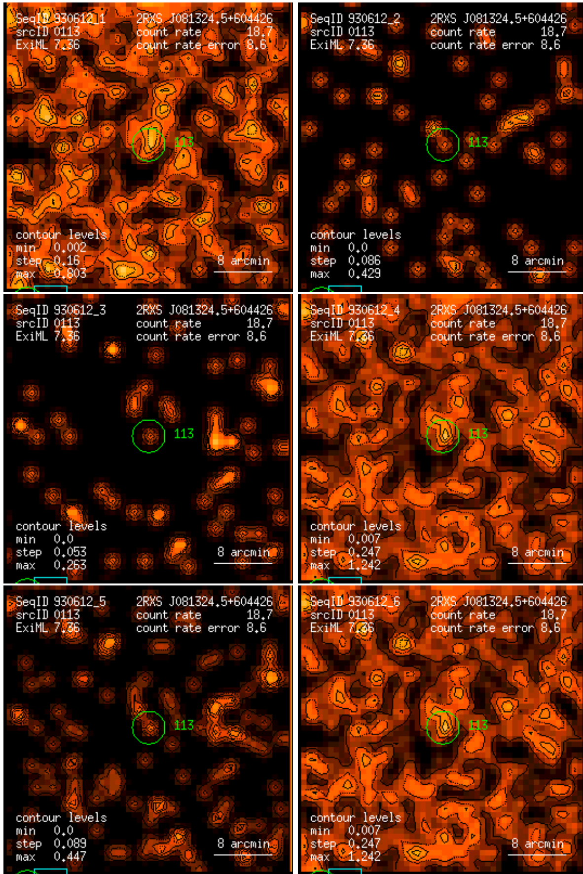
Figure 113: RASS 930612: detection 0113: band rate images, Gaussian filter: (1) PSPC channels 11 – 41, (2) 52 – 90, (3) 91 – 201, (4) 11 – 235, (5) 52 – 201, (6) 11 – 201. Broad band rates in counts/ks. Band rate contour levels in counts/ks/arcmin 2 .
