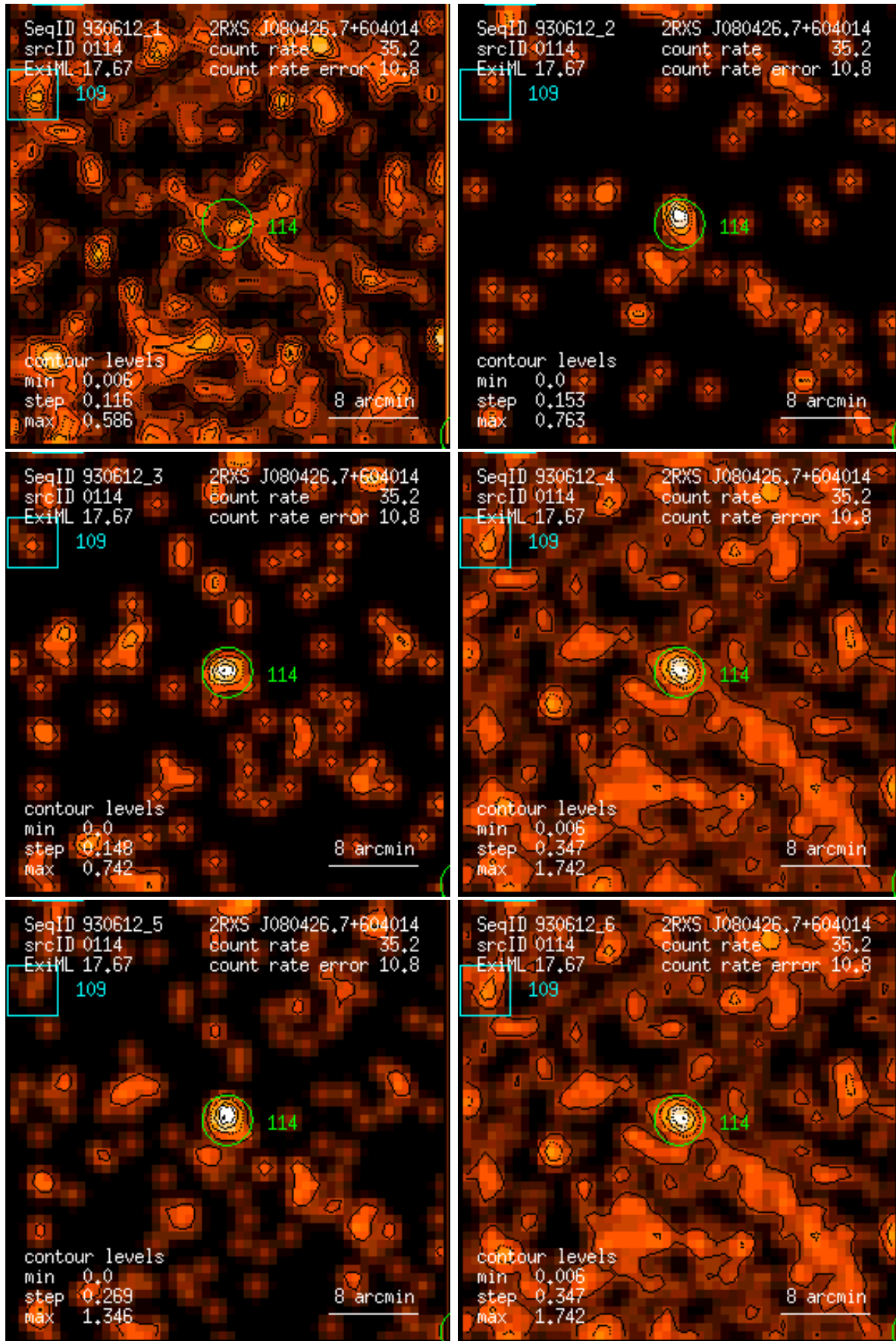
Figure 114: RASS 930612: detection 0114: band rate images, Gaussian filter: (1) PSPC channels 11 – 41, (2) 52 – 90, (3) 91 – 201, (4) 11 – 235, (5) 52 – 201, (6) 11 – 201. Broad band rates in counts/ks. Band rate contour levels in counts/ks/arcmin 2 .
