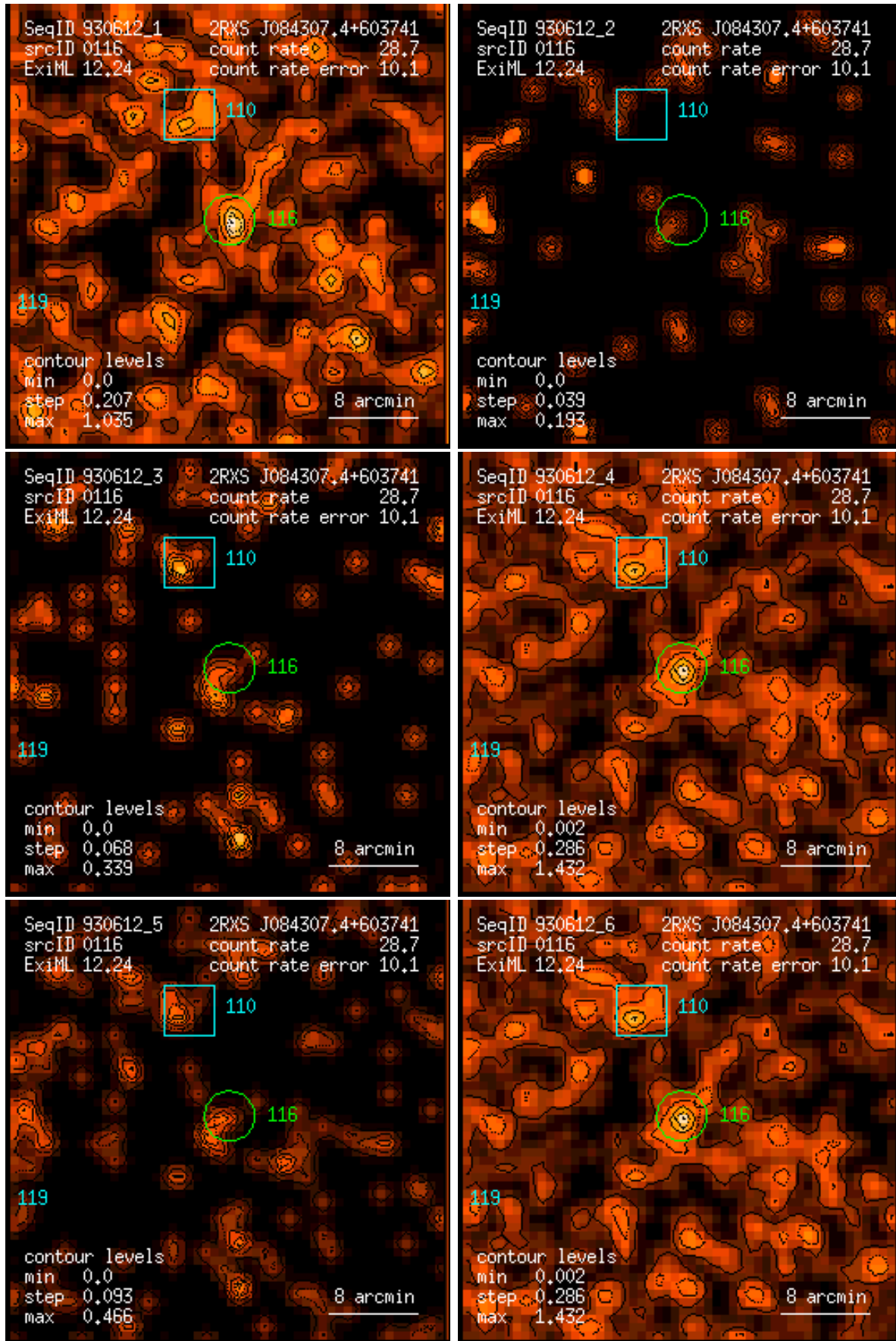
Figure 116: RASS 930612: detection 0116: band rate images, Gaussian filter: (1) PSPC channels 11 – 41, (2) 52 – 90, (3) 91 – 201, (4) 11 – 235, (5) 52 – 201, (6) 11 – 201. Broad band rates in counts/ks. Band rate contour levels in counts/ks/arcmin 2 .
