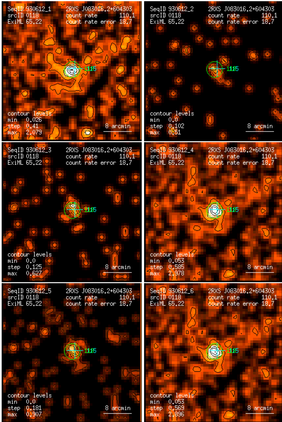
Figure 118: RASS 930612: detection 0118: band rate images, Gaussian filter: (1) PSPC channels 11 – 41, (2) 52 – 90, (3) 91 – 201, (4) 11 – 235, (5) 52 – 201, (6) 11 – 201. Broad band rates in counts/ks. Band rate contour levels in counts/ks/arcmin 2 .
