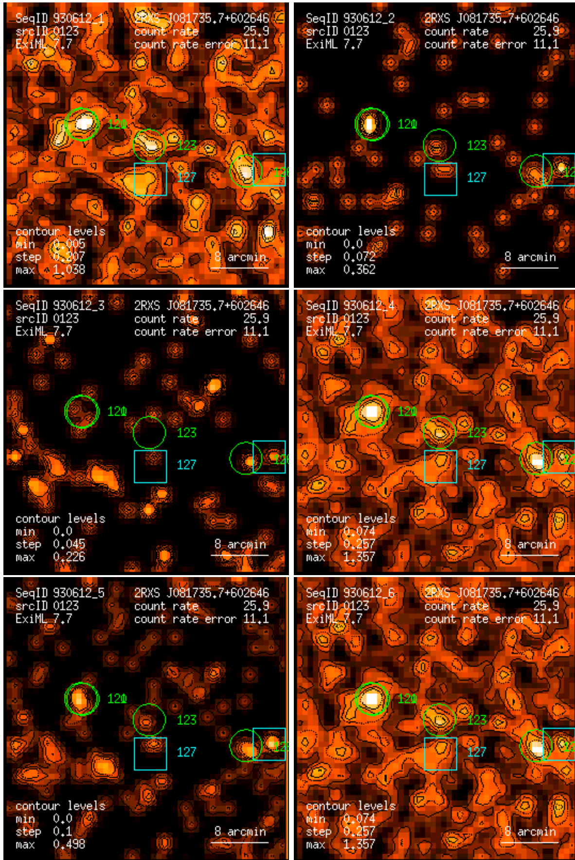
Figure 123: RASS 930612: detection 0123: band rate images, Gaussian filter: (1) PSPC channels 11 – 41, (2) 52 – 90, (3) 91 – 201, (4) 11 – 235, (5) 52 – 201, (6) 11 – 201. Broad band rates in counts/ks. Band rate contour levels in counts/ks/arcmin 2 .
