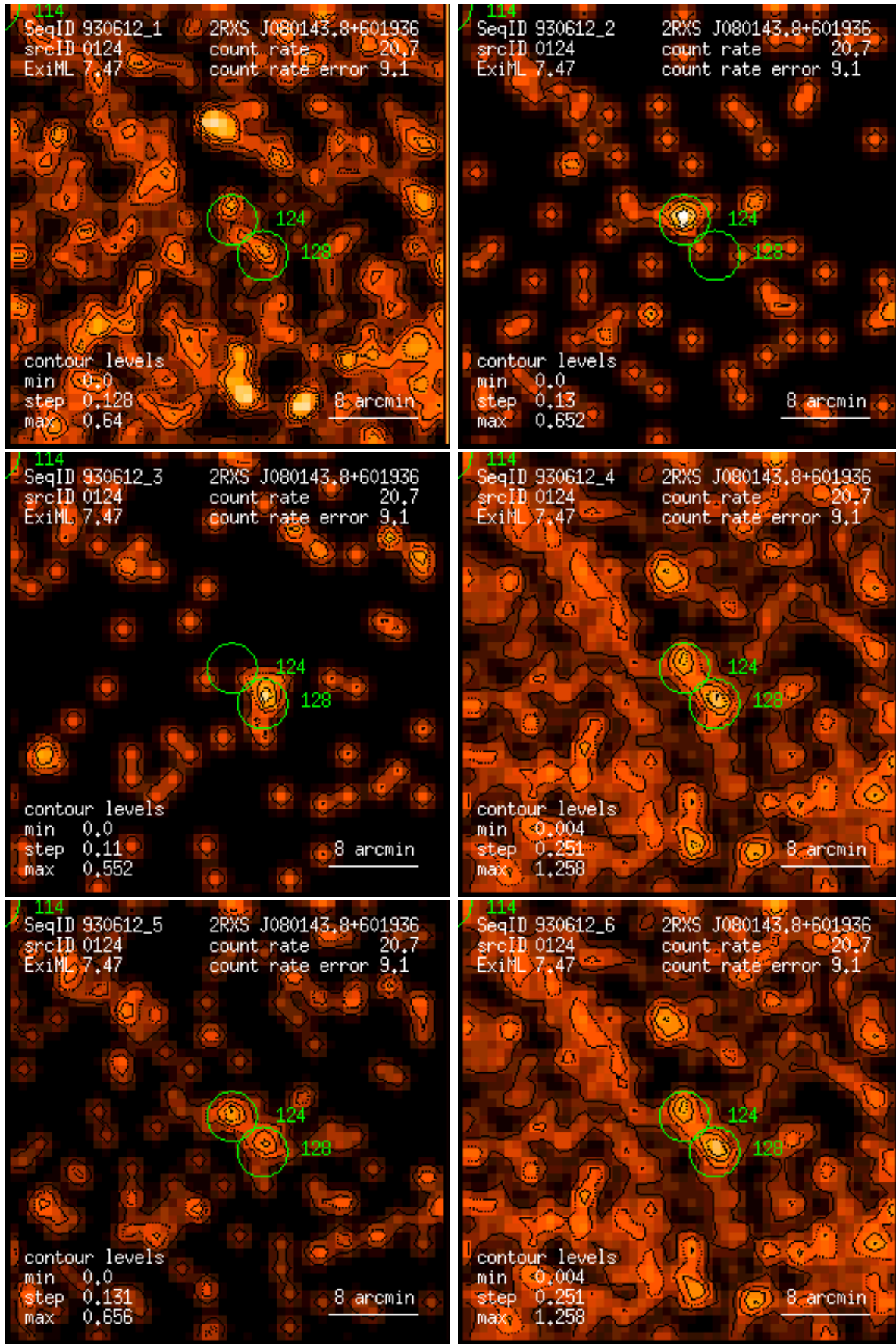
Figure 124: RASS 930612: detection 0124: band rate images, Gaussian filter: (1) PSPC channels 11 – 41, (2) 52 – 90, (3) 91 – 201, (4) 11 – 235, (5) 52 – 201, (6) 11 – 201. Broad band rates in counts/ks. Band rate contour levels in counts/ks/arcmin 2 .
