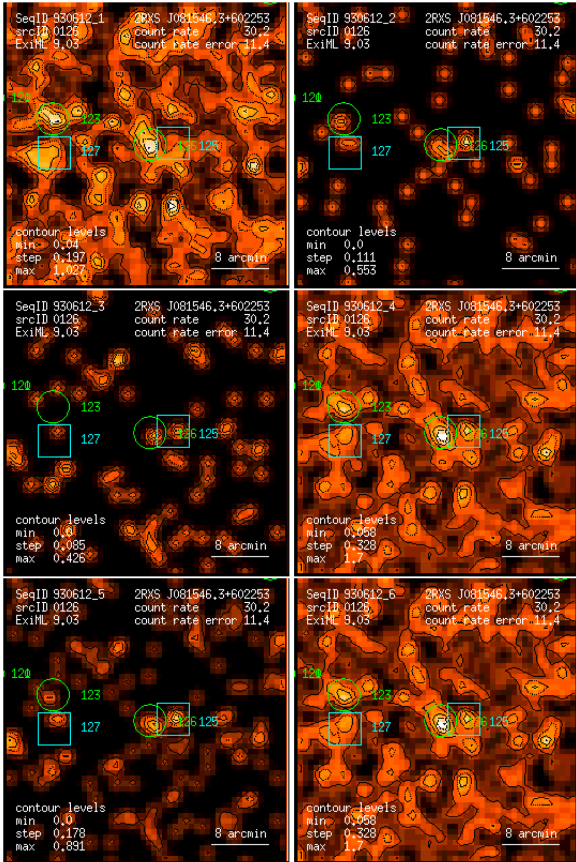
Figure 126: RASS 930612: detection 0126: band rate images, Gaussian filter: (1) PSPC channels 11 – 41, (2) 52 – 90, (3) 91 – 201, (4) 11 – 235, (5) 52 – 201, (6) 11 – 201. Broad band rates in counts/ks. Band rate contour levels in counts/ks/arcmin 2 .
