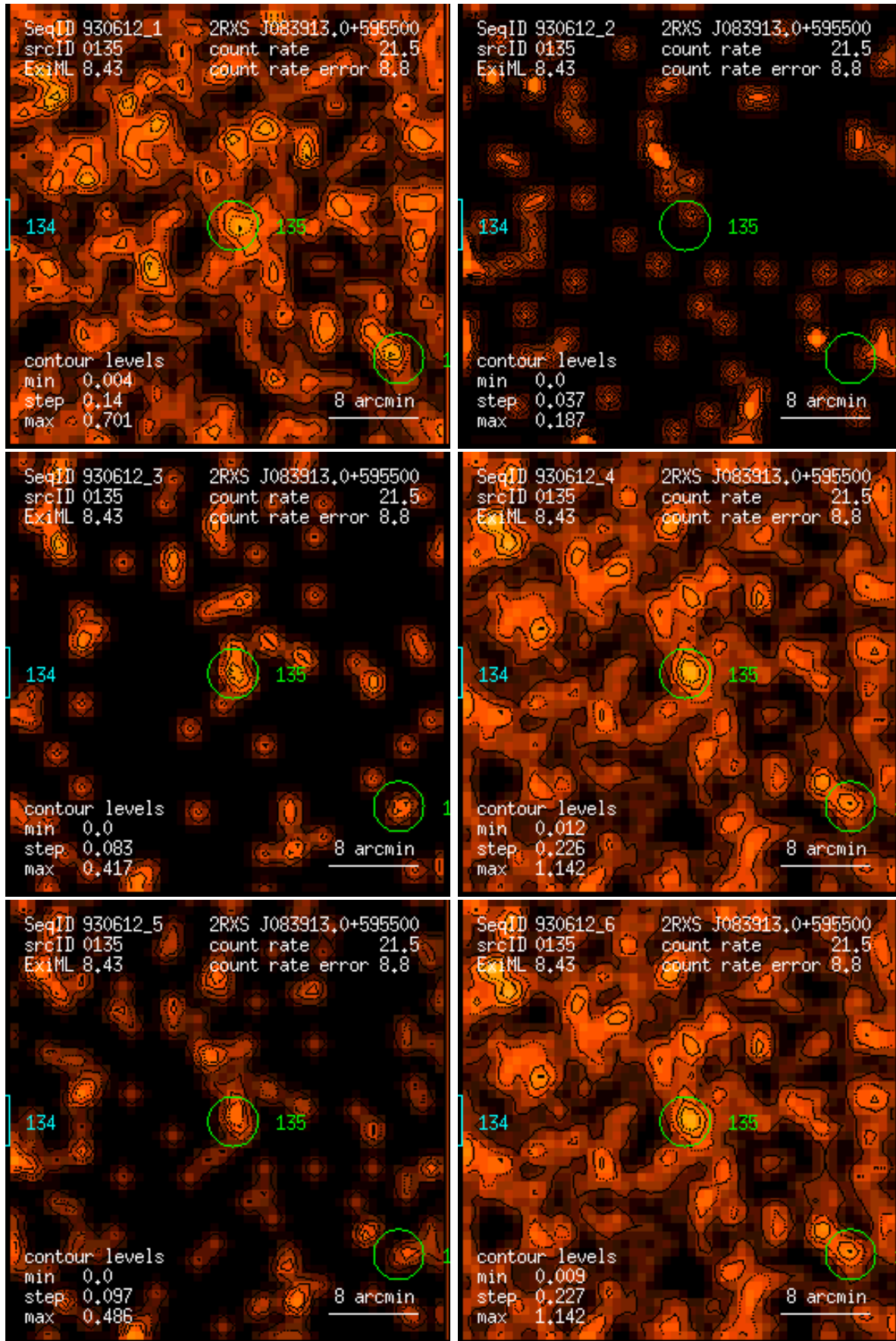
Figure 135: RASS 930612: detection 0135: band rate images, Gaussian filter: (1) PSPC channels 11 – 41, (2) 52 – 90, (3) 91 – 201, (4) 11 – 235, (5) 52 – 201, (6) 11 – 201. Broad band rates in counts/ks. Band rate contour levels in counts/ks/arcmin 2 .
