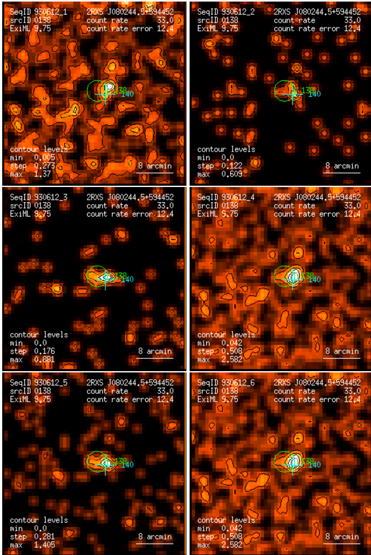
Figure 138: RASS 930612: detection 0138: band rate images, Gaussian filter: (1) PSPC channels 11 – 41, (2) 52 – 90, (3) 91 – 201, (4) 11 – 235, (5) 52 – 201, (6) 11 – 201. Broad band rates in counts/ks. Band rate contour levels in counts/ks/arcmin 2 .
