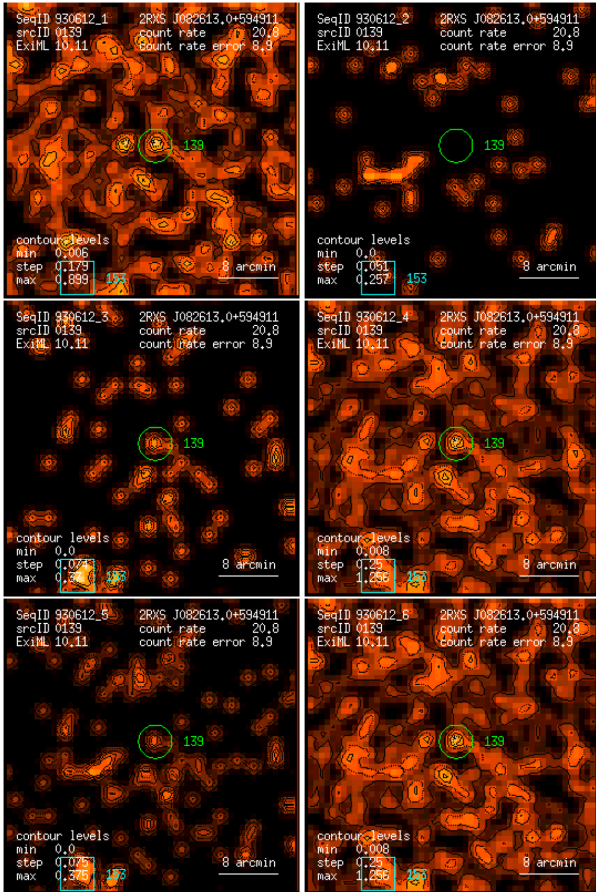
Figure 139: RASS 930612: detection 0139: band rate images, Gaussian filter: (1) PSPC channels 11 – 41, (2) 52 – 90, (3) 91 – 201, (4) 11 – 235, (5) 52 – 201, (6) 11 – 201. Broad band rates in counts/ks. Band rate contour levels in counts/ks/arcmin 2 .
