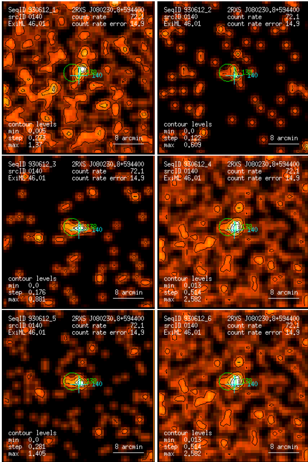
Figure 140: RASS 930612: detection 0140: band rate images, Gaussian filter: (1) PSPC channels 11 – 41, (2) 52 – 90, (3) 91 – 201, (4) 11 – 235, (5) 52 – 201, (6) 11 – 201. Broad band rates in counts/ks. Band rate contour levels in counts/ks/arcmin 2 .
