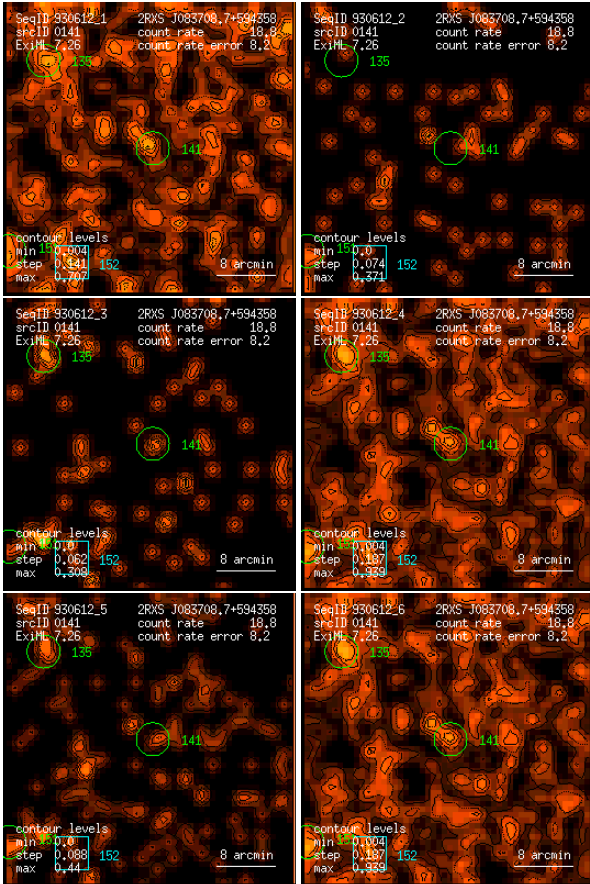
Figure 141: RASS 930612: detection 0141: band rate images, Gaussian filter: (1) PSPC channels 11 – 41, (2) 52 – 90, (3) 91 – 201, (4) 11 – 235, (5) 52 – 201, (6) 11 – 201. Broad band rates in counts/ks. Band rate contour levels in counts/ks/arcmin 2 .
