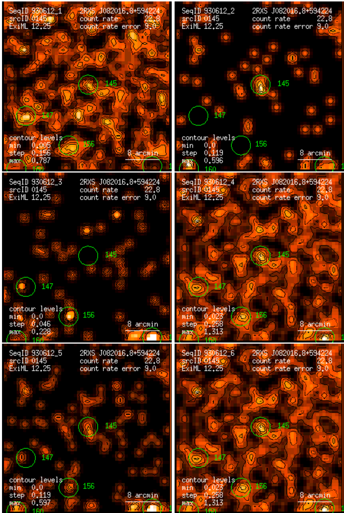
Figure 145: RASS 930612: detection 0145: band rate images, Gaussian filter: (1) PSPC channels 11 – 41, (2) 52 – 90, (3) 91 – 201, (4) 11 – 235, (5) 52 – 201, (6) 11 – 201. Broad band rates in counts/ks. Band rate contour levels in counts/ks/arcmin 2 .
