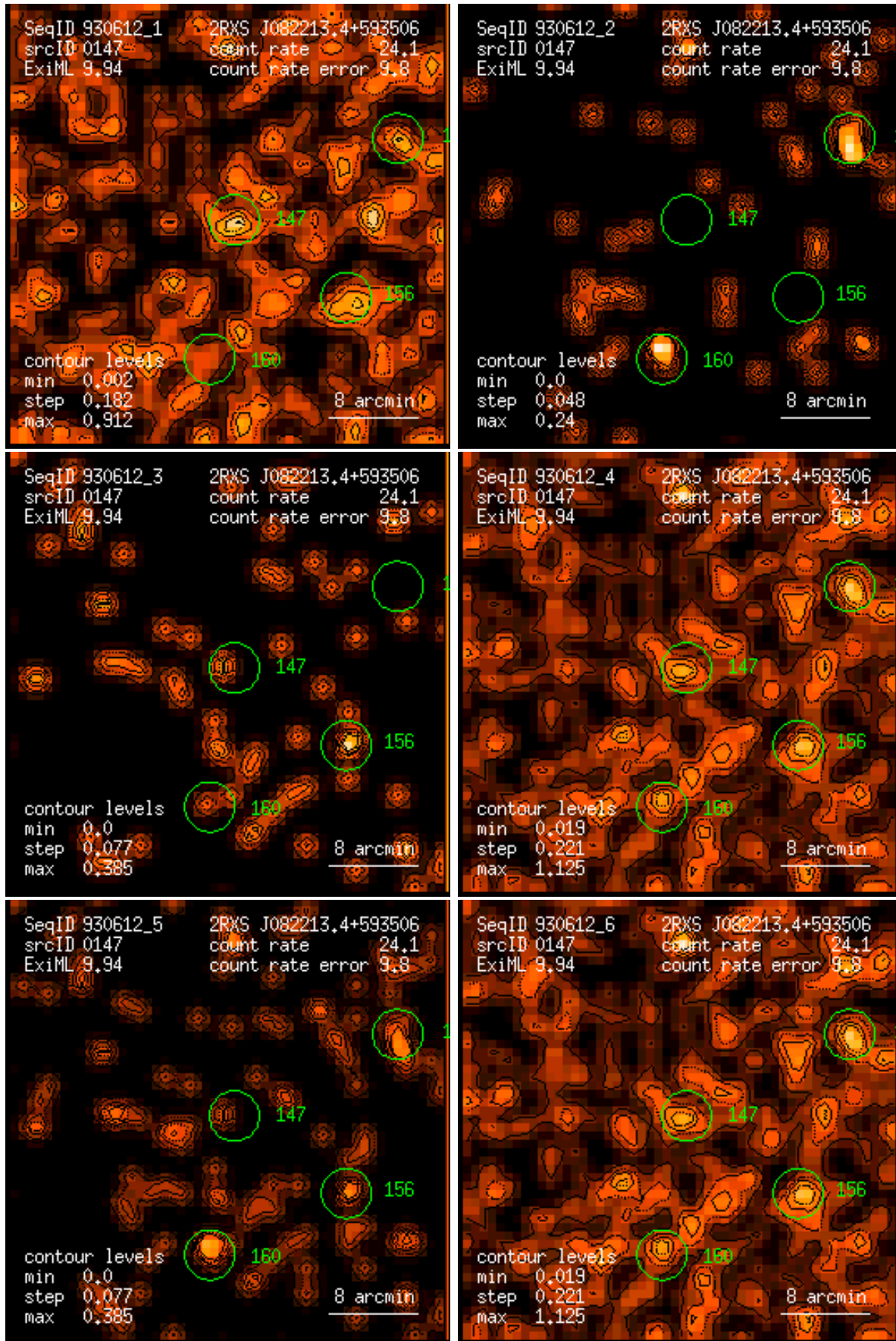
Figure 147: RASS 930612: detection 0147: band rate images, Gaussian filter: (1) PSPC channels 11 – 41, (2) 52 – 90, (3) 91 – 201, (4) 11 – 235, (5) 52 – 201, (6) 11 – 201. Broad band rates in counts/ks. Band rate contour levels in counts/ks/arcmin 2 .
