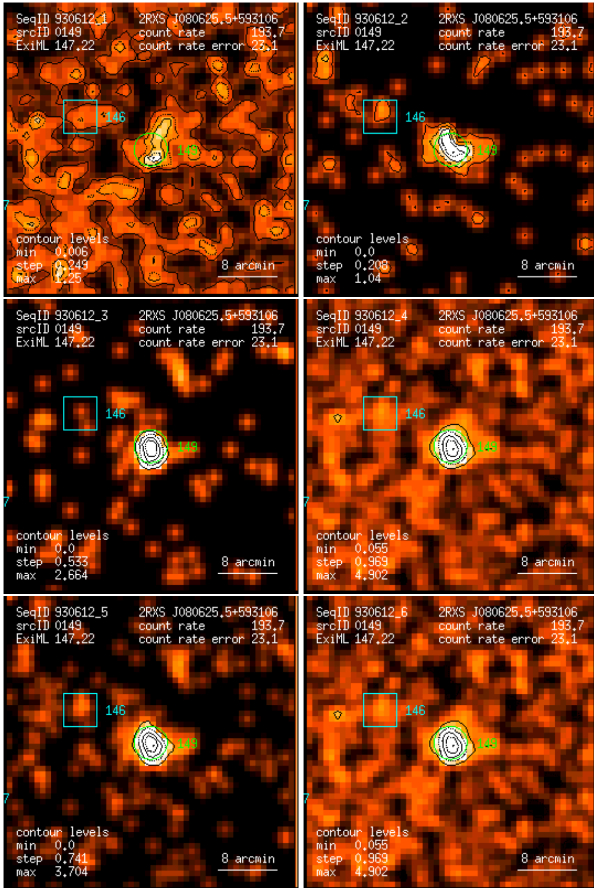
Figure 149: RASS 930612: detection 0149: band rate images, Gaussian filter: (1) PSPC channels 11 – 41, (2) 52 – 90, (3) 91 – 201, (4) 11 – 235, (5) 52 – 201, (6) 11 – 201. Broad band rates in counts/ks. Band rate contour levels in counts/ks/arcmin 2 .
