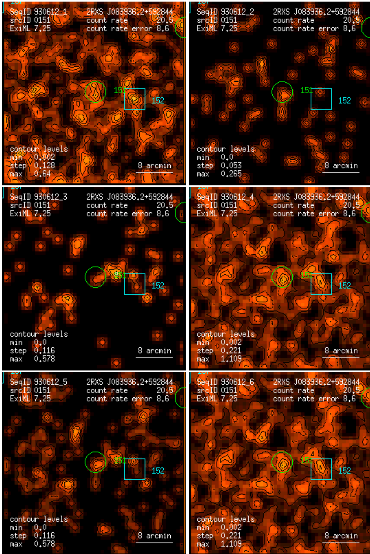
Figure 151: RASS 930612: detection 0151: band rate images, Gaussian filter: (1) PSPC channels 11 – 41, (2) 52 – 90, (3) 91 – 201, (4) 11 – 235, (5) 52 – 201, (6) 11 – 201. Broad band rates in counts/ks. Band rate contour levels in counts/ks/arcmin 2 .
