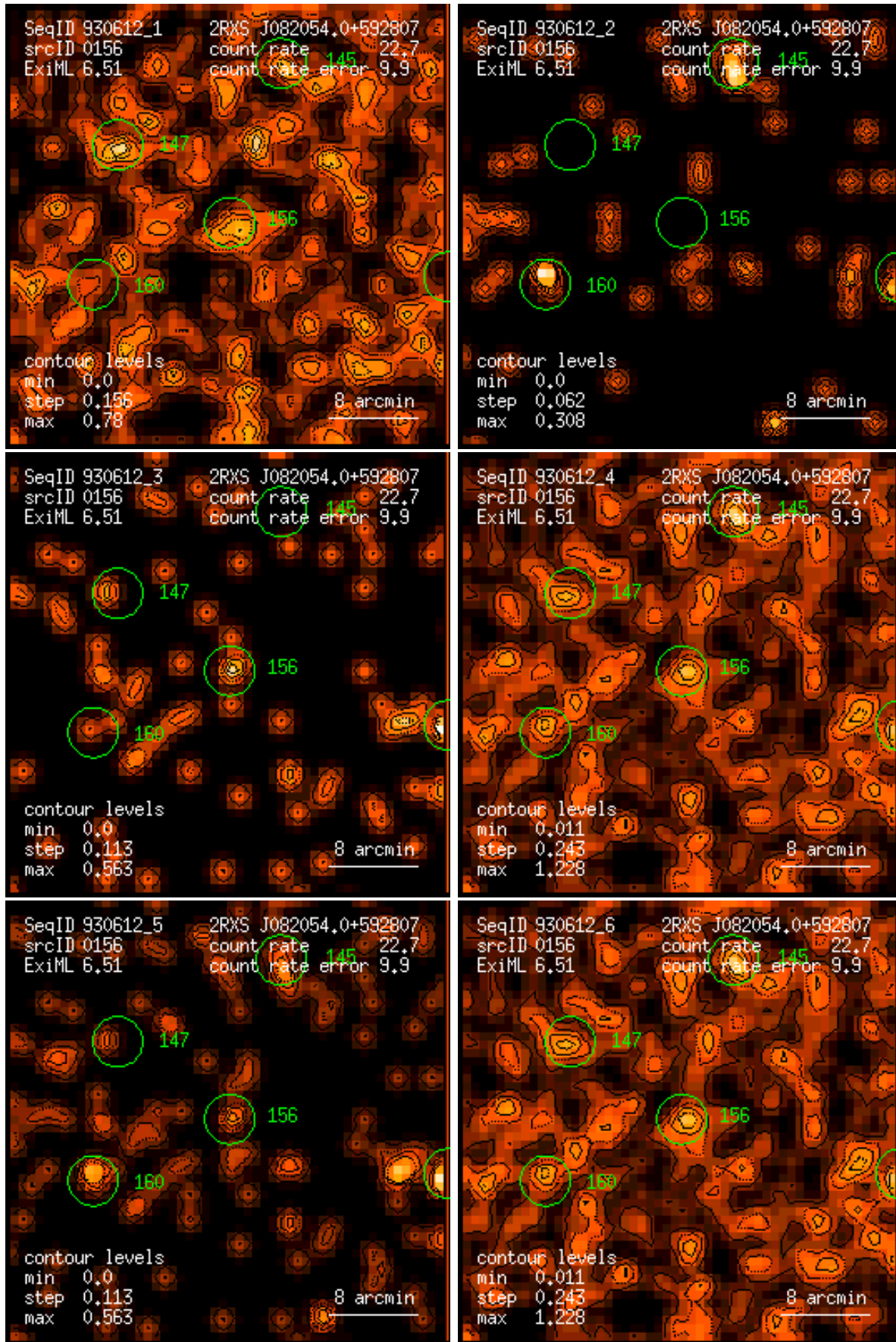
Figure 156: RASS 930612: detection 0156: band rate images, Gaussian filter: (1) PSPC channels 11 – 41, (2) 52 – 90, (3) 91 – 201, (4) 11 – 235, (5) 52 – 201, (6) 11 – 201. Broad band rates in counts/ks. Band rate contour levels in counts/ks/arcmin 2 .
