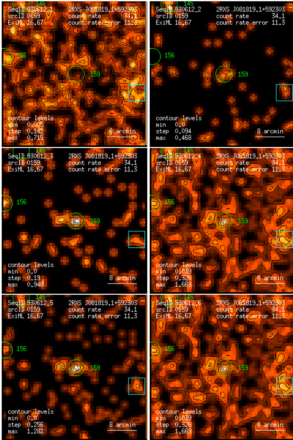
Figure 159: RASS 930612: detection 0159: band rate images, Gaussian filter: (1) PSPC channels 11 – 41, (2) 52 – 90, (3) 91 – 201, (4) 11 – 235, (5) 52 – 201, (6) 11 – 201. Broad band rates in counts/ks. Band rate contour levels in counts/ks/arcmin 2 .
