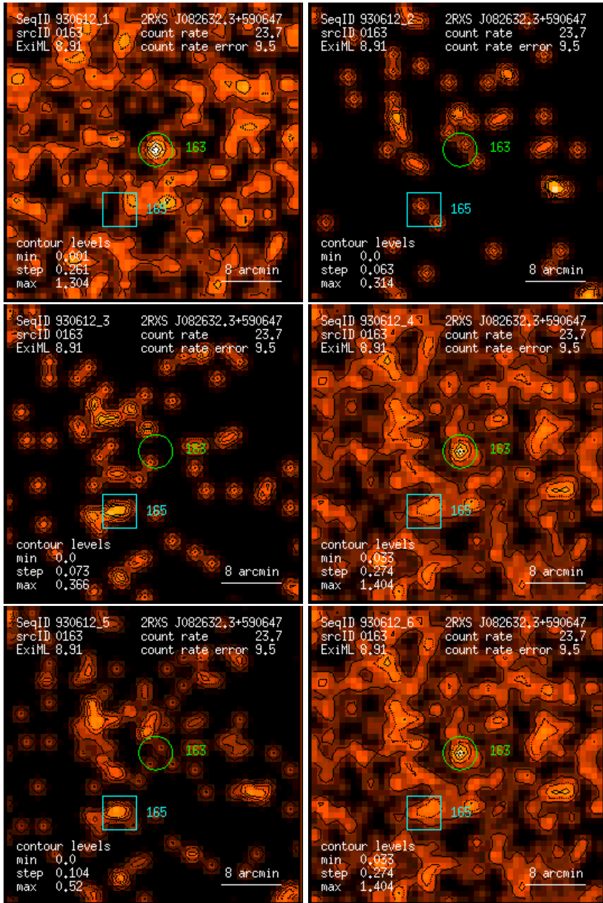
Figure 163: RASS 930612: detection 0163: band rate images, Gaussian filter: (1) PSPC channels 11 – 41, (2) 52 – 90, (3) 91 – 201, (4) 11 – 235, (5) 52 – 201, (6) 11 – 201. Broad band rates in counts/ks. Band rate contour levels in counts/ks/arcmin 2 .
