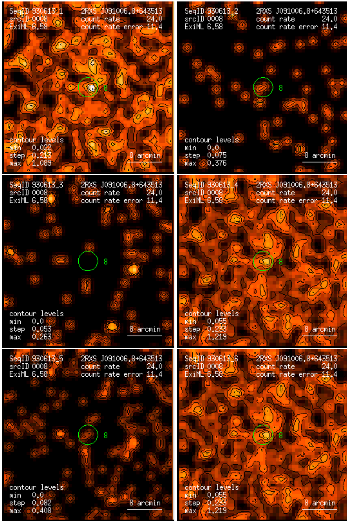
Figure 8: RASS 930613: detection 0008: band rate images, Gaussian filter: (1) PSPC channels 11 – 41, (2) 52 – 90, (3) 91 – 201, (4) 11 – 235, (5) 52 – 201, (6) 11 – 201. Broad band rates in counts/ks. Band rate contour levels in counts/ks/arcmin 2 .
