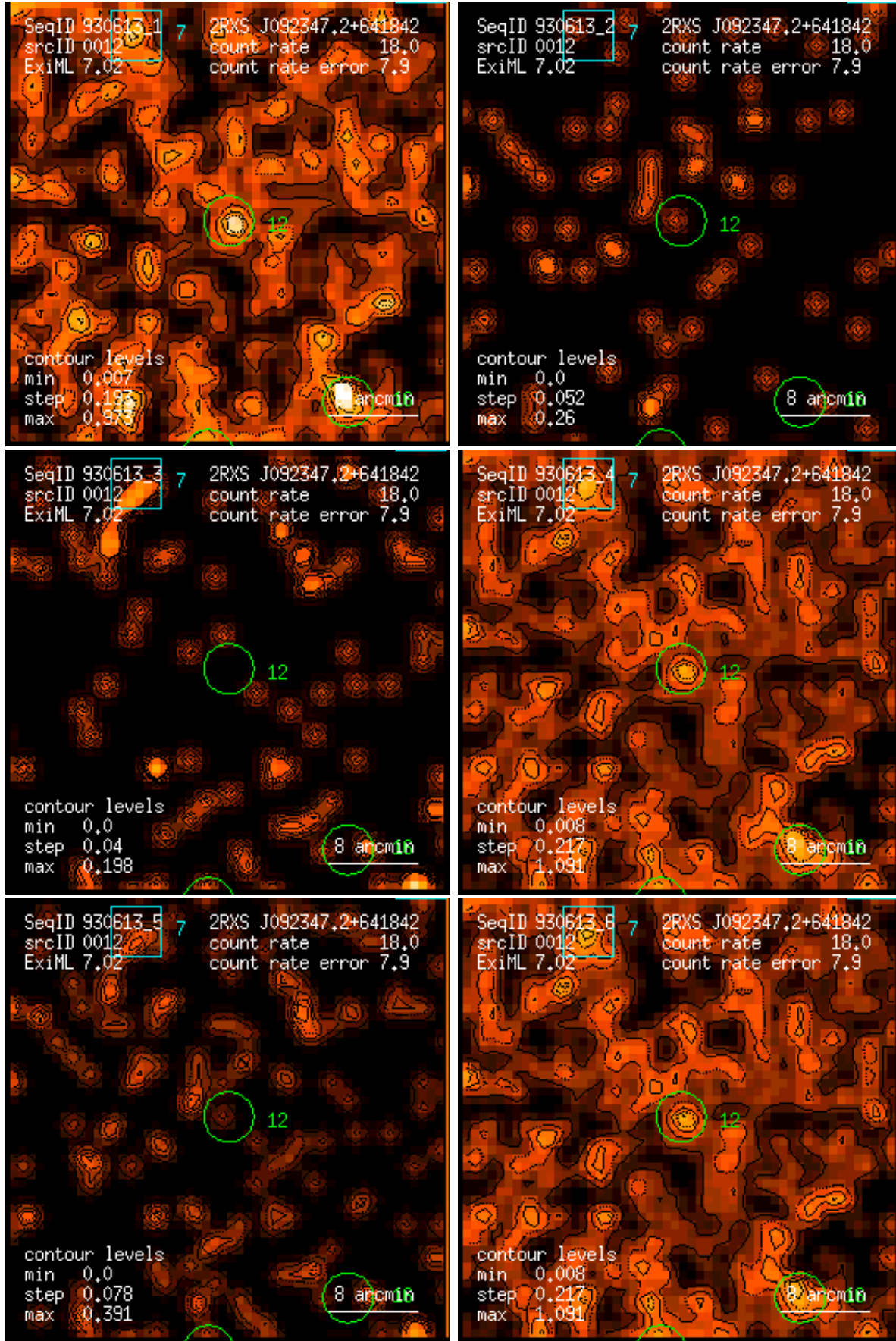
Figure 12: RASS 930613: detection 0012: band rate images, Gaussian filter: (1) PSPC channels 11 – 41, (2) 52 – 90, (3) 91 – 201, (4) 11 – 235, (5) 52 – 201, (6) 11 – 201. Broad band rates in counts/ks. Band rate contour levels in counts/ks/arcmin 2 .
