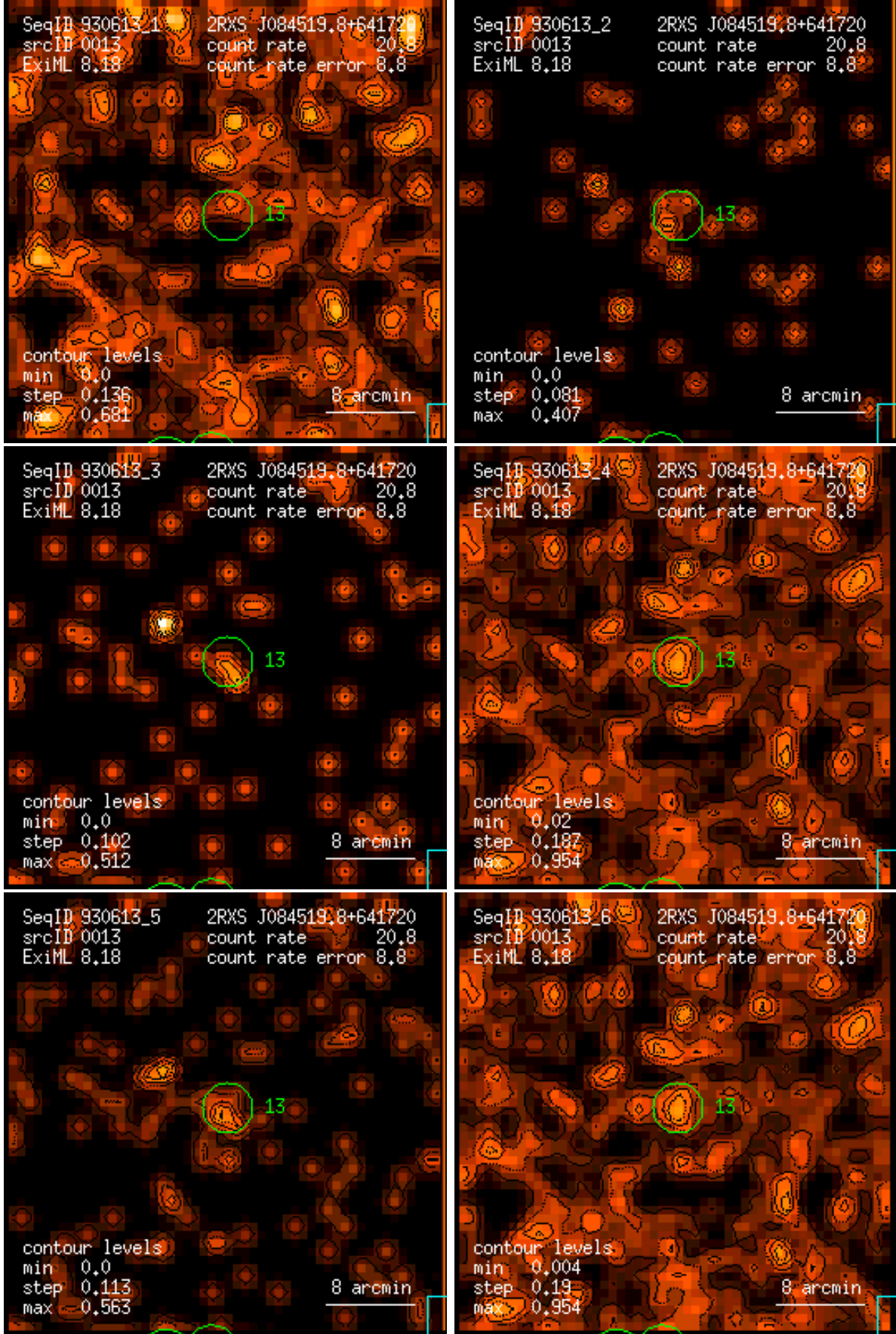
Figure 13: RASS 930613: detection 0013: band rate images, Gaussian filter: (1) PSPC channels 11 – 41, (2) 52 – 90, (3) 91 – 201, (4) 11 – 235, (5) 52 – 201, (6) 11 – 201. Broad band rates in counts/ks. Band rate contour levels in counts/ks/arcmin 2 .
