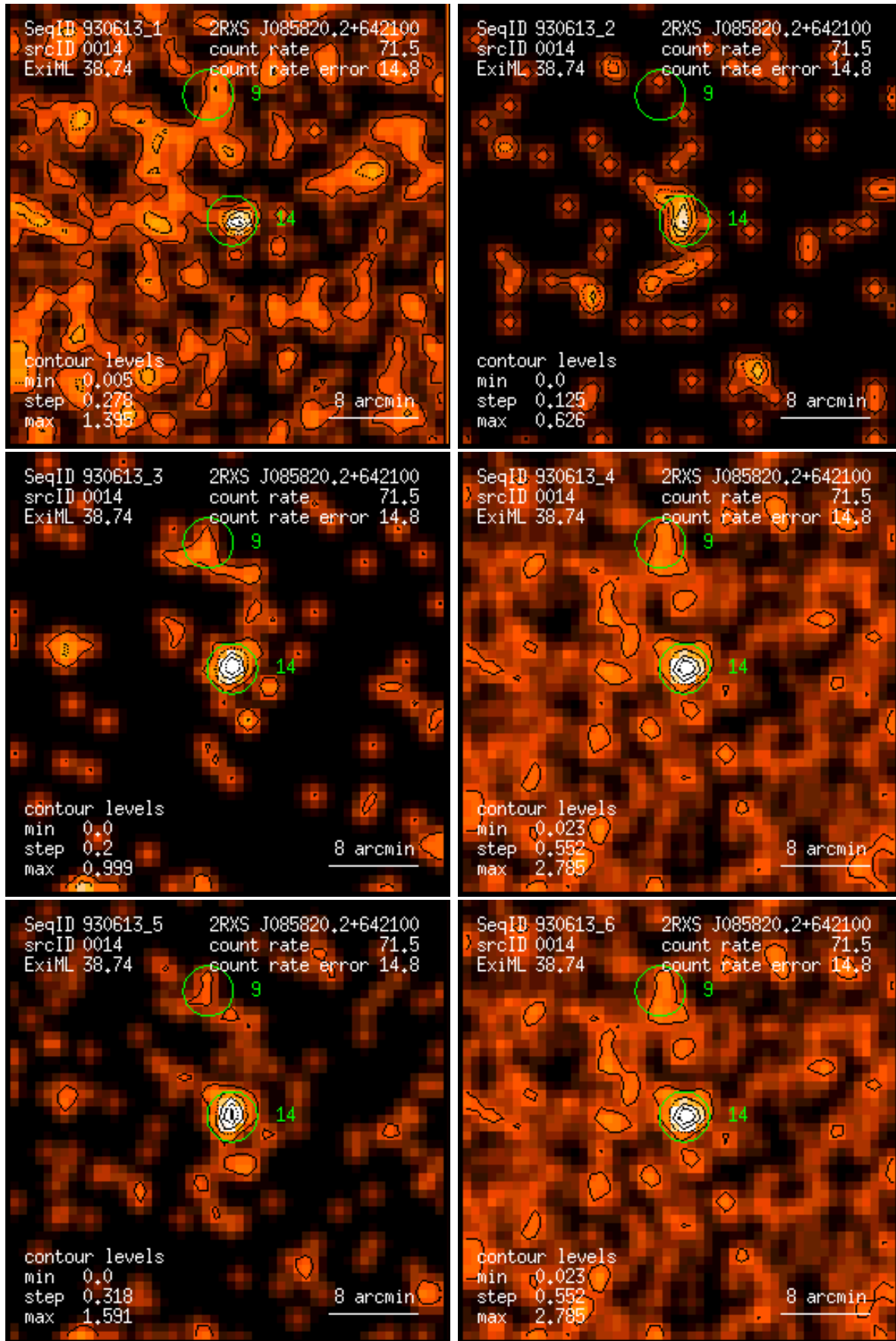
Figure 14: RASS 930613: detection 0014: band rate images, Gaussian filter: (1) PSPC channels 11 – 41, (2) 52 – 90, (3) 91 – 201, (4) 11 – 235, (5) 52 – 201, (6) 11 – 201. Broad band rates in counts/ks. Band rate contour levels in counts/ks/arcmin 2 .
